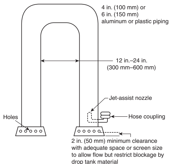
FIGURE C.11.2.3(a) Jet-Assist Transfer Siphon.
