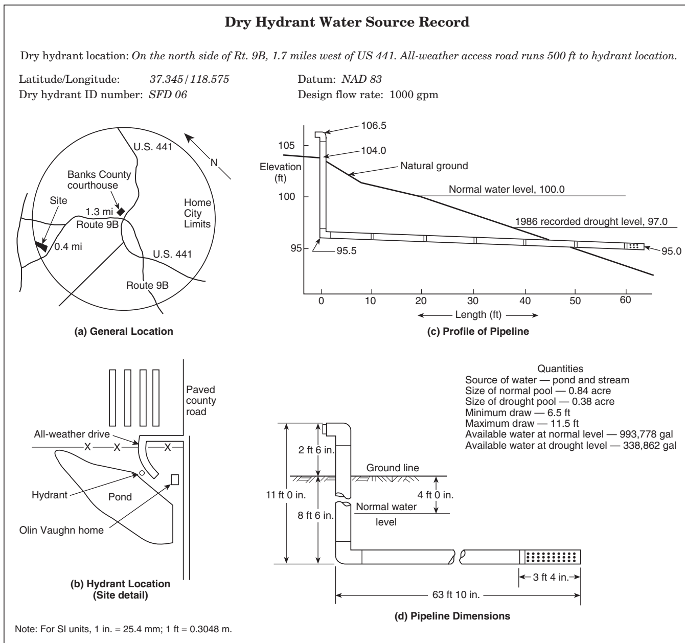
FIGURE A.8.8(a) Example of Dry Hydrant Water Source Record.
