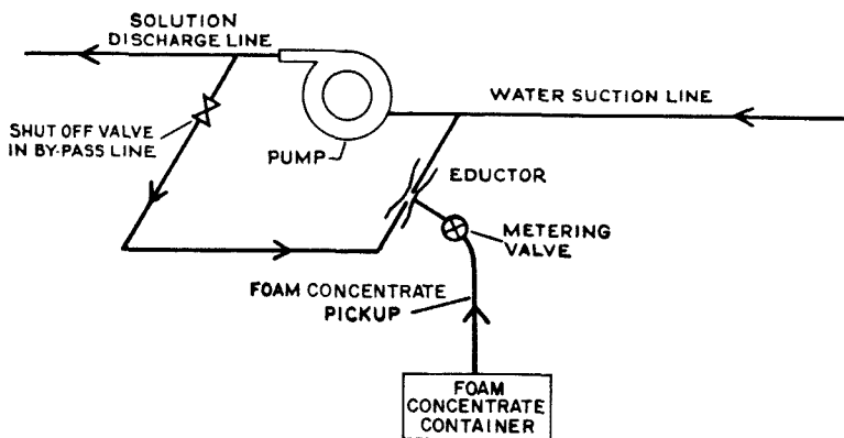
Fig. A-121(c). Around-the-Pump Proportioner.
