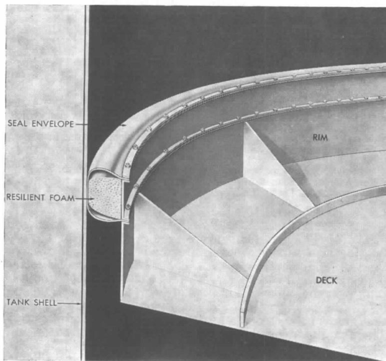
Fig. A-3312. Seal on floating metal pan of covered floating roof tank.
