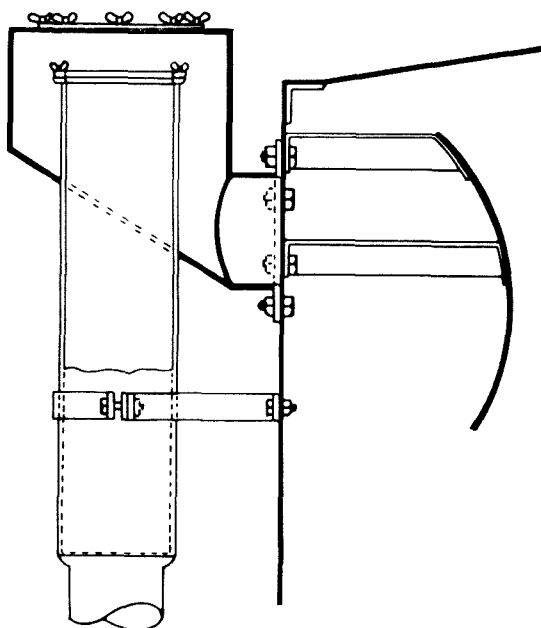
Figure A-302(c). Air Foam Chamber with Type II Outlet.
