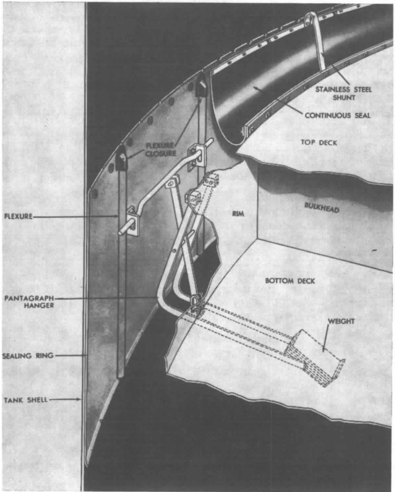
Fig. A-3311(1). Pantograph type seal-open top floating roof tank.
