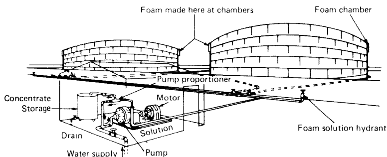
Fig. A-300. Schematic arrangement of air foam protection for storage tanks.
