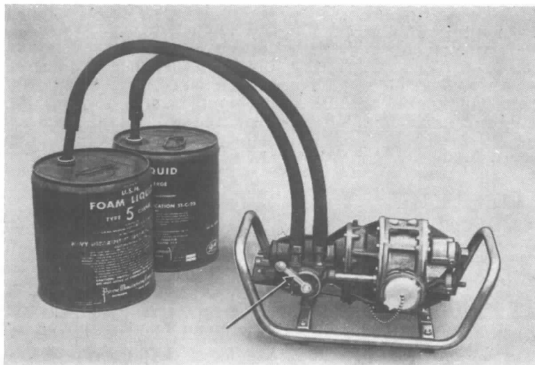
Fig. A-121(f). Coupled water motor pump proportioner.
