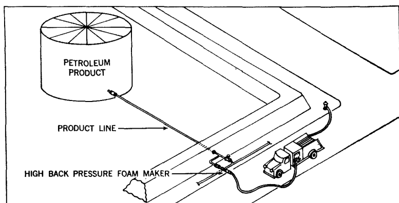
Fig. A-302(d). Semi-fixed subsurface foam installation.
