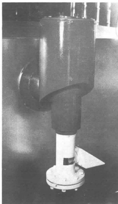
Fig. A-331 (b). Foam chamber and foam maker.
