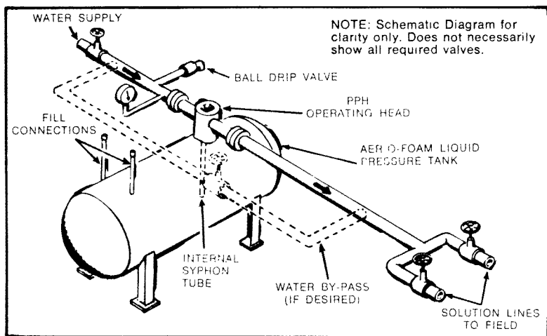
Fig. A-121(e). Typical arrangement of pressure proportioner with single operating head.
