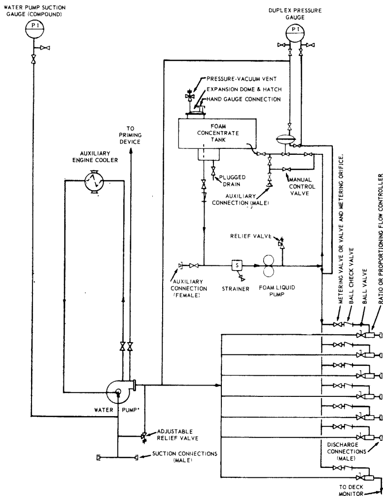
Fig. A-121(d). Balanced pressure proportioning.
