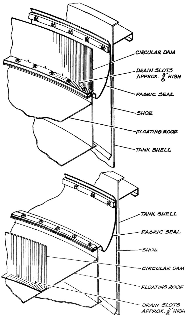
Fig. A-3311 (3). Typical Foam Dams for Floating Roof Tank Fixed Protection.
