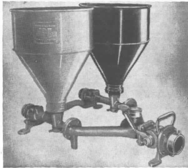
Figure A-131(a). Dual Hopper Chemical Foam generator of the two powder type.
