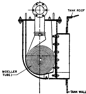
Fig. A-302 (b) (1). Cross-section Moeller Tube Chamber. Tube is designed to unroll and fall to oil level. Foam flows through interstices in tube.
