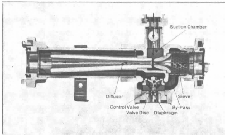
Fig. A-121(b)(1)(b). In-Line Inductor.
