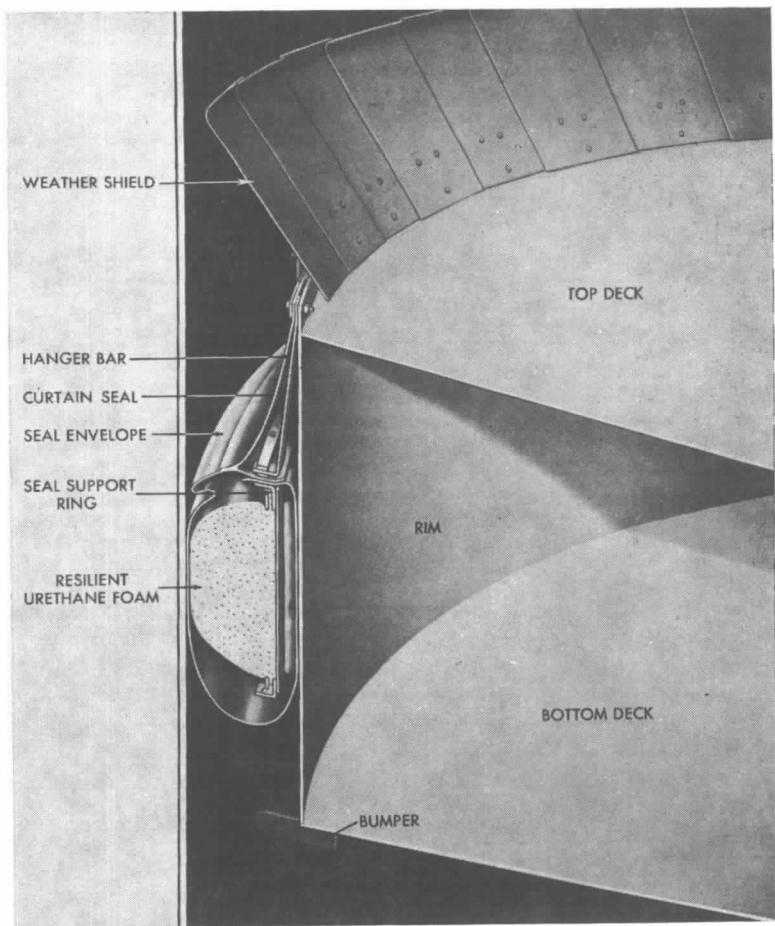
Fig. A-3311 (2). Tube seal-open floating roof tank.
