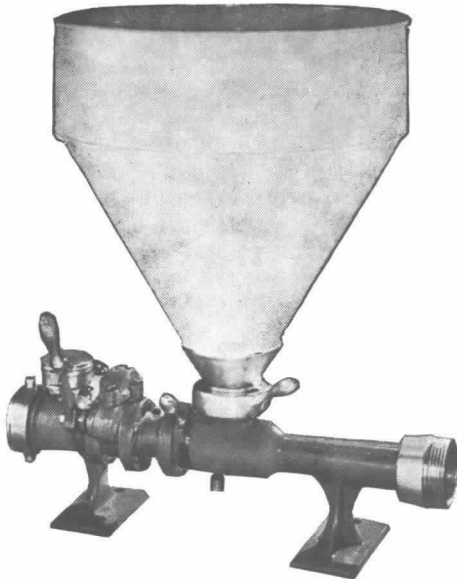
Figure A-131(b). Single Hopper Chemical Foam generator of the single powder type.
