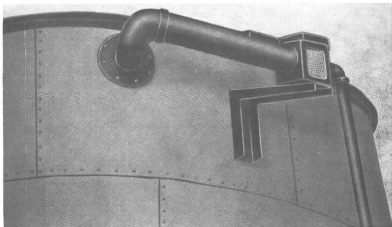
Fig. A-331 (a). Air Foam Maker in Horizontal Position at Top of Storage Tank.
