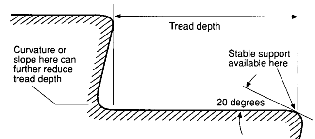
Figure A-5-2.2.2.3(d) Tread measurement with stable support at leading edge.
