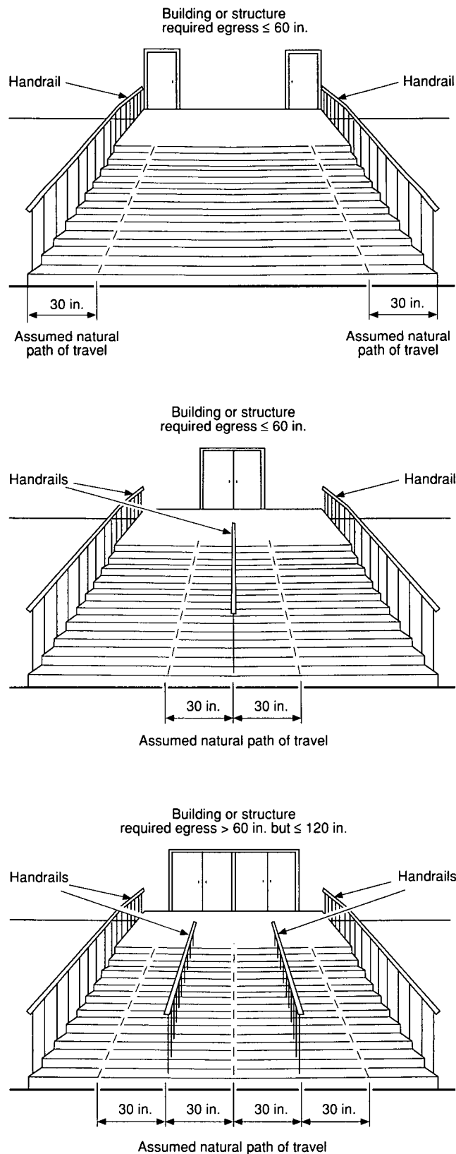
Figure A-5-2.2.4.2 Assumed natural paths of travel on monumental stairs with various handrail locations.
