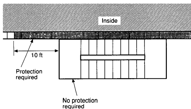
Figure A-5-2.2.6.2(b) Stairway with unprotected exterior perimeter protruding past building exterior wall.
