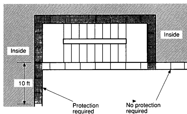
Figure A-5-2.2.6.2(c) Stairway with nonrated exterior wall exposed by adjacent exterior wall of building.
