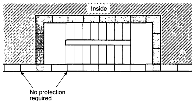
Figure A-5-2.2.6.2(a) Stairway with nonrated exterior wall in same plane as building exterior wall.
