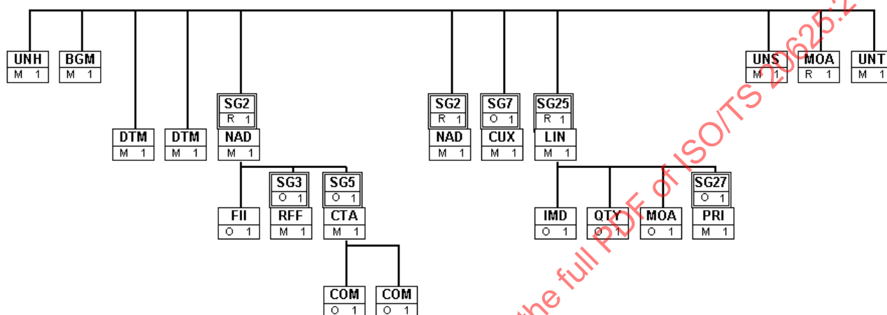
Figure A.1 — Message structure diagram (Branching Diagram) of the based EDIFACT ORDERS
