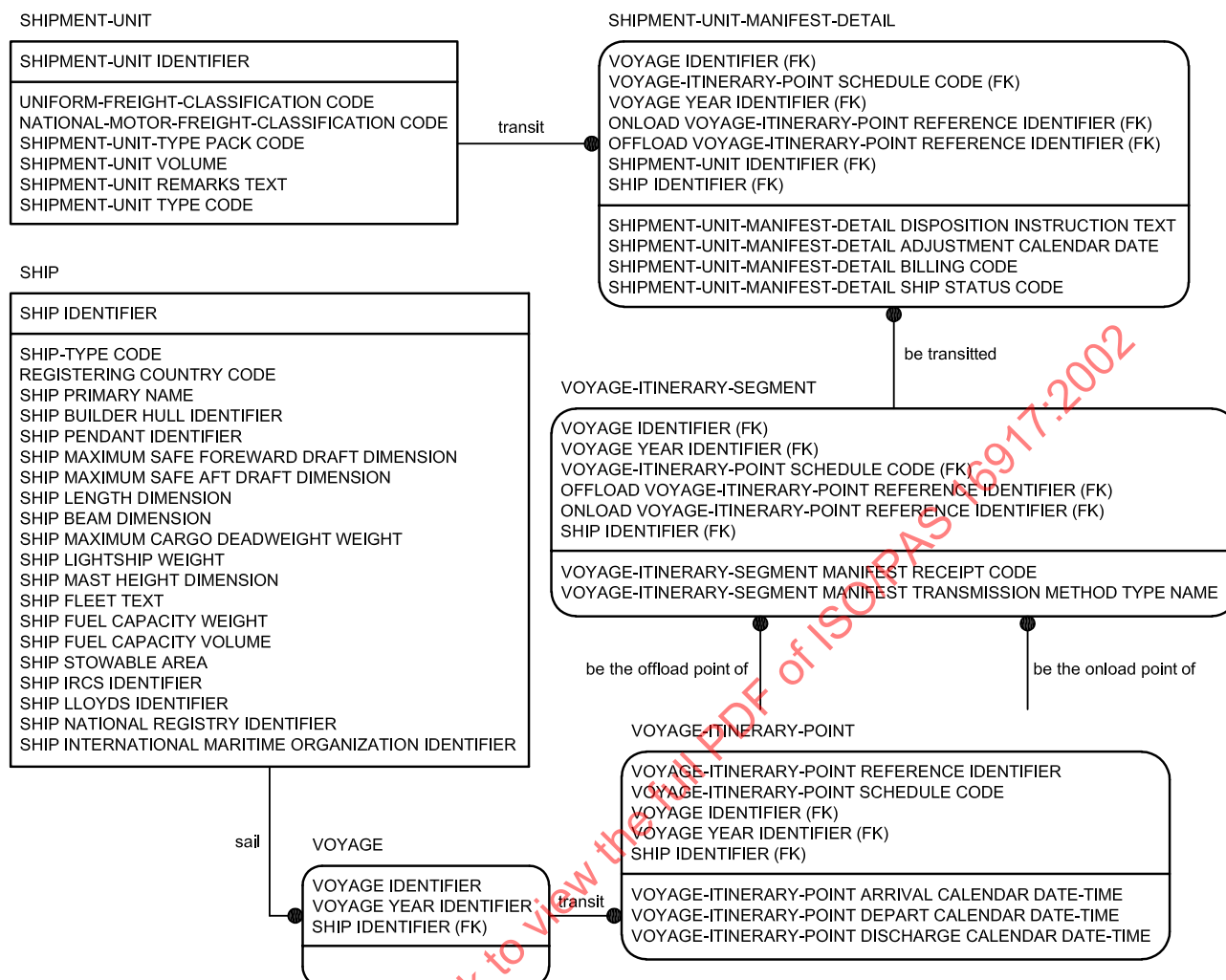
Figure 4 — Example of a portion of application-domain model
