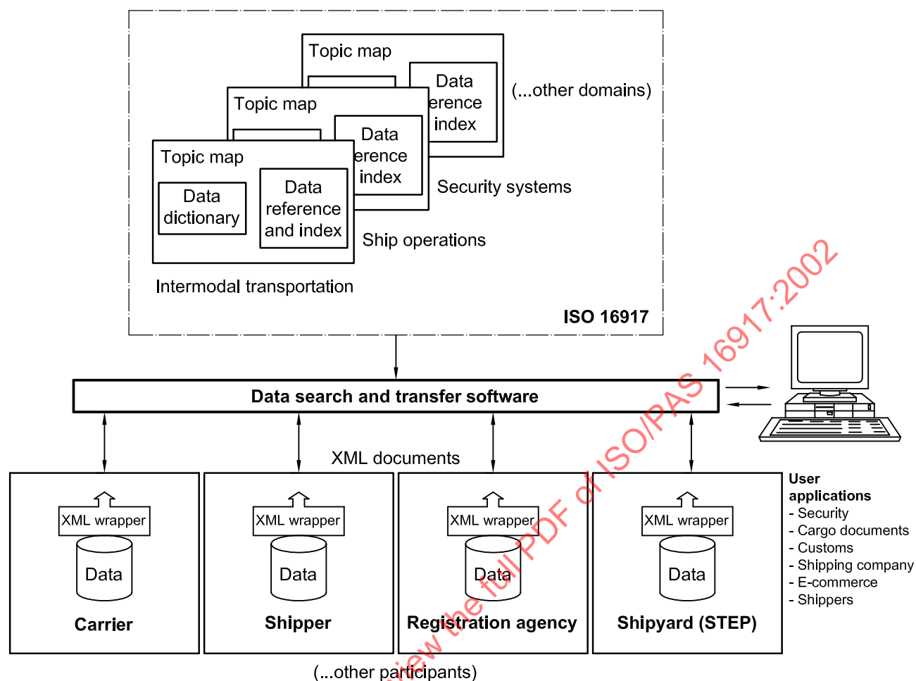
Figure 5 — Architecture of data-transfer standard
