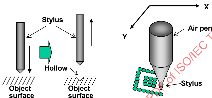
Figure A.4 — Dot peen marking
