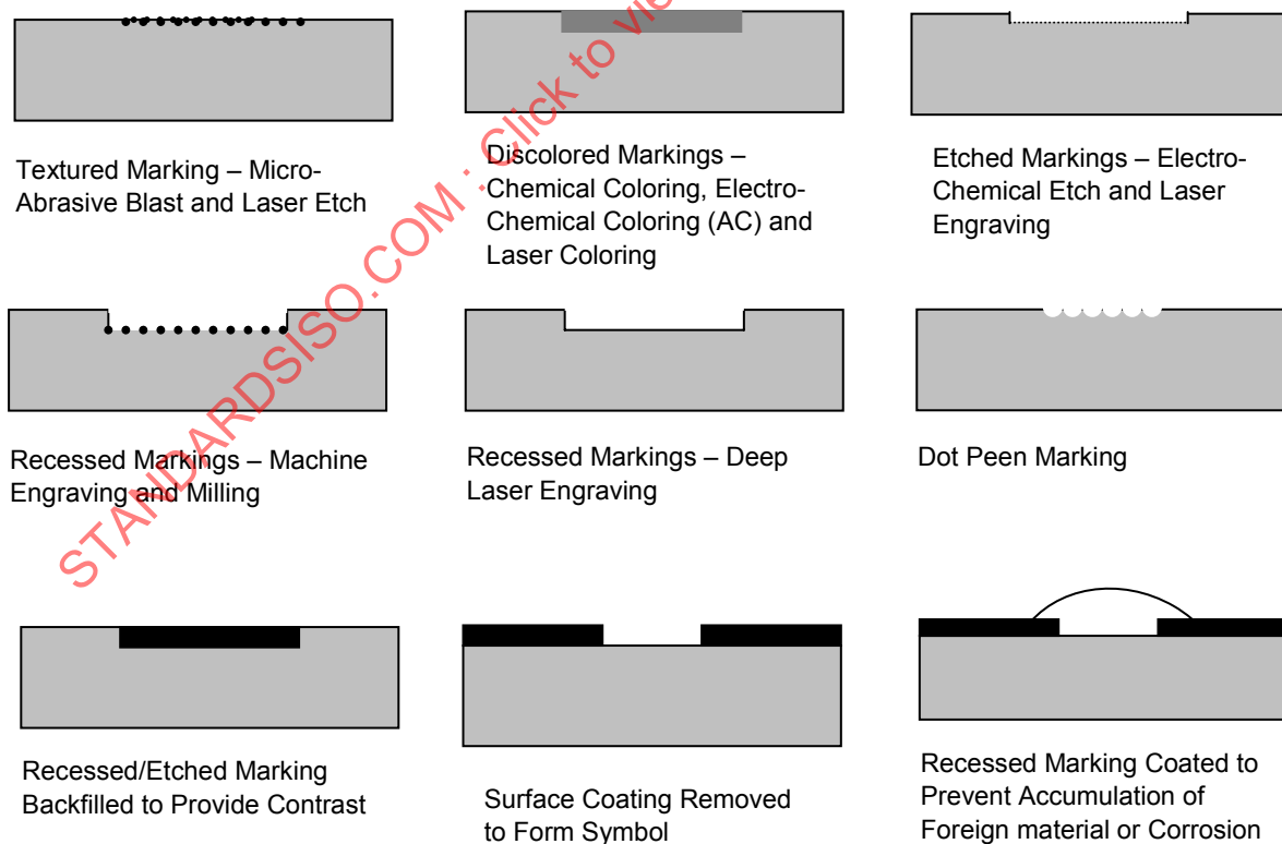
Figure A.1 — Intrusive marking cross-sections
