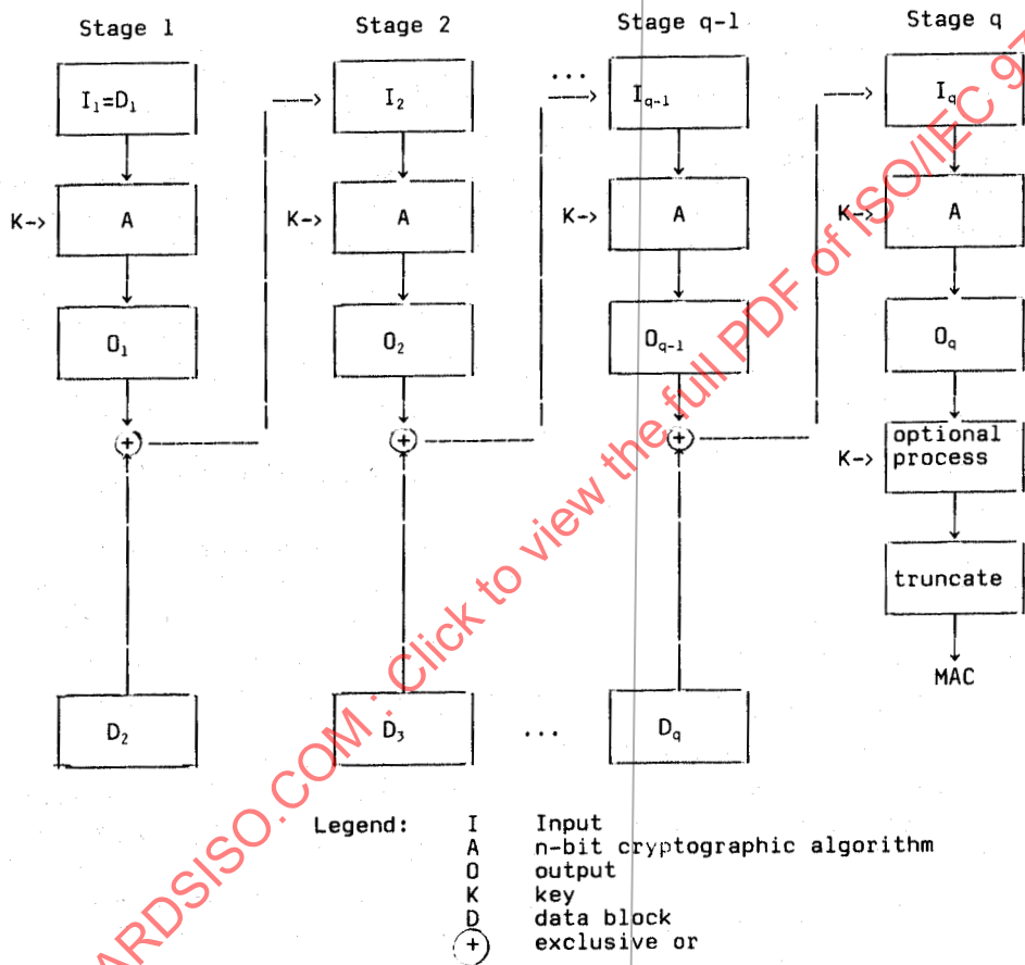
Figure 1 – The MAC calculation
