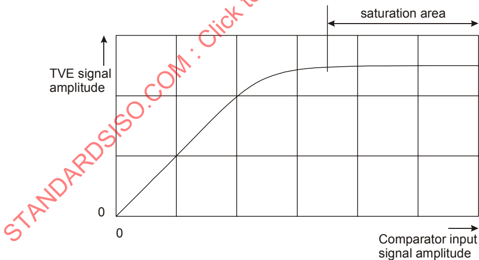
Figure F.2 — Tracking error signal amplitude versus comparator input signal amplitude
