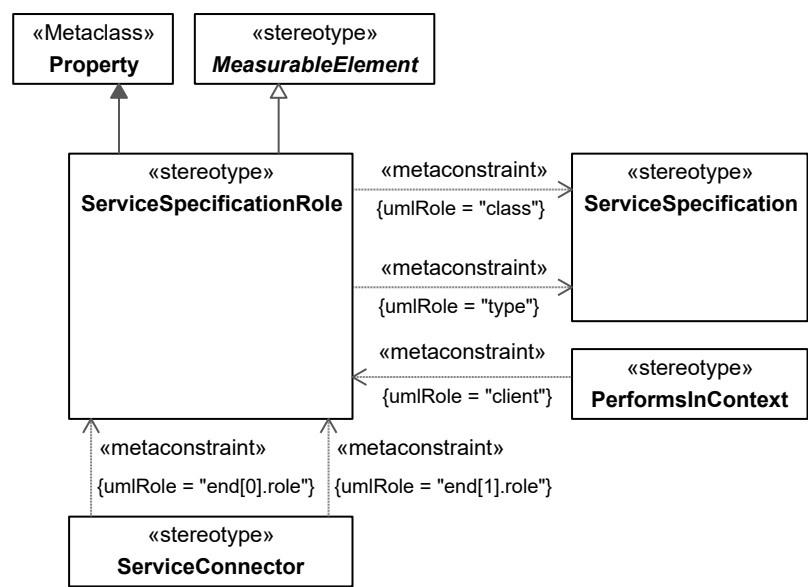
Figure 3:89 – ServiceSpecificationRole
