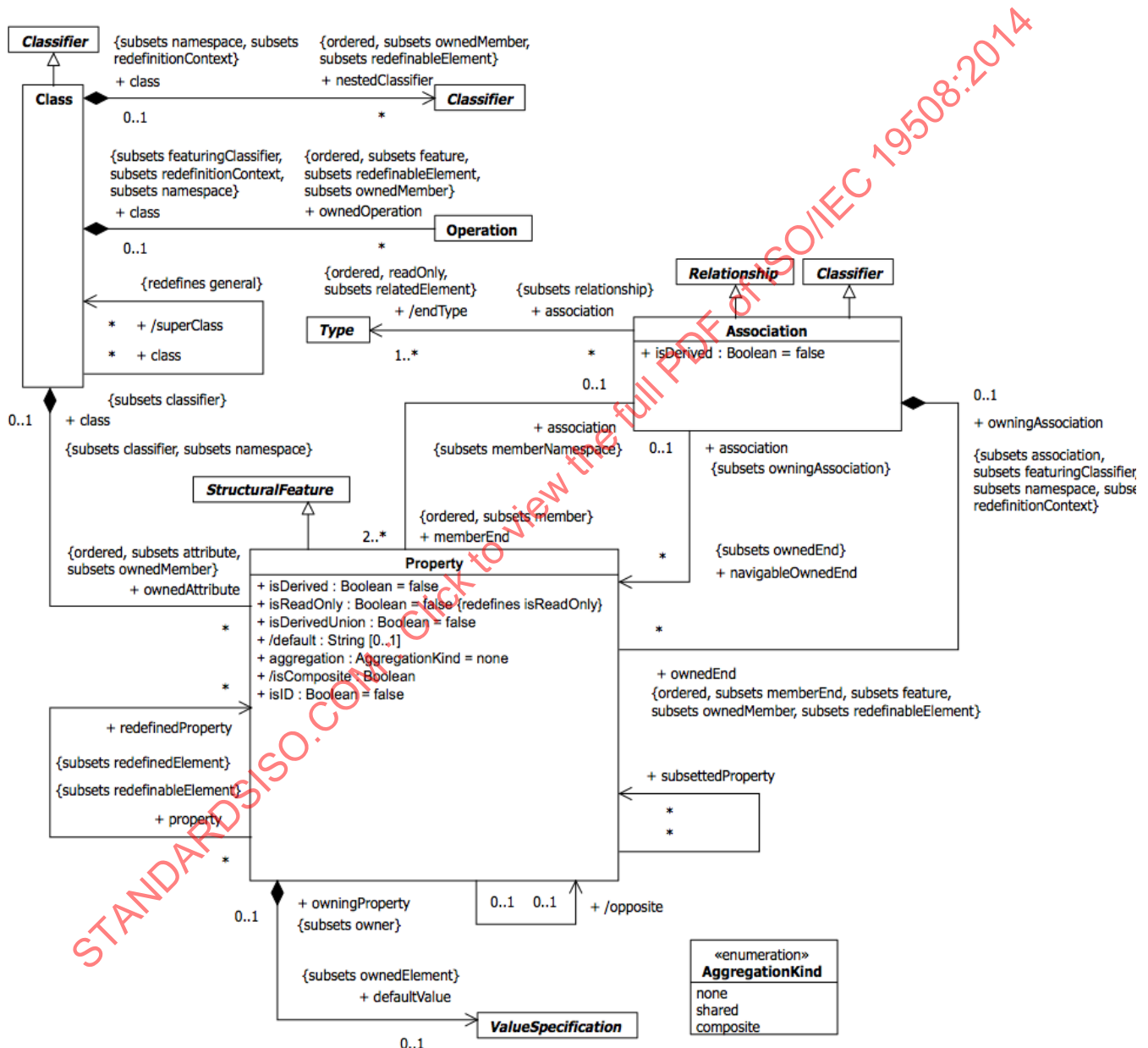
Figure 14.2 - Key concrete classes from UML2 Kernel package
