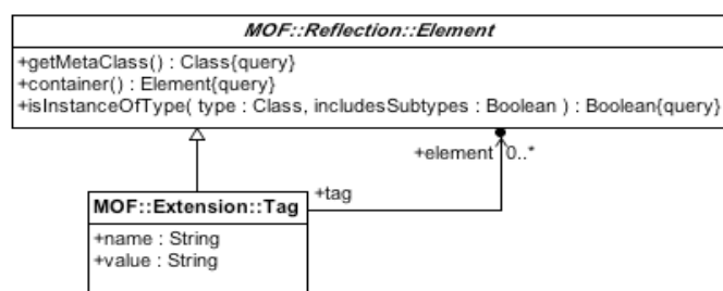
Figure 11.1 - The Extension package
