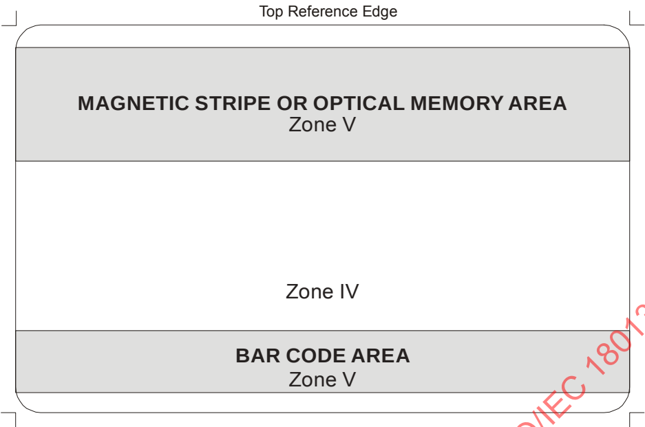
Figure A.6 — Non-portrait side of IDL – magnetic stripe or optical memory and bar code (not to scale)
