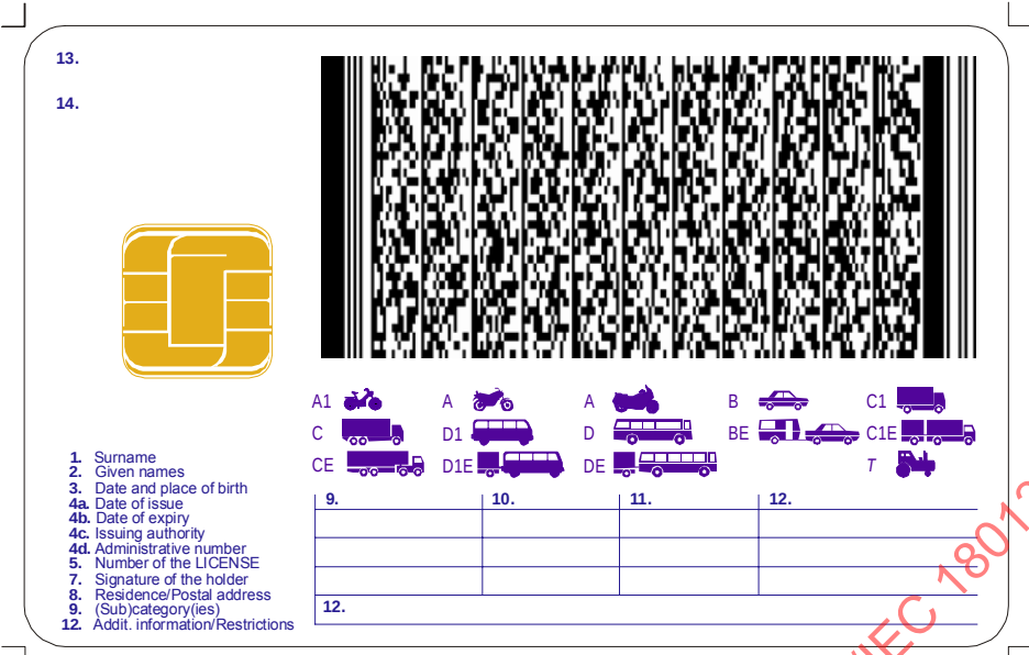
Figure A.7.1 — Informative example (not to scale)
