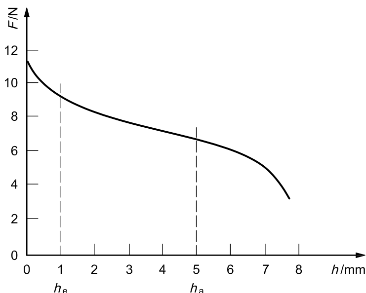
Figure A.2 — Solenoid characteristics for a plunger stroke of 4 mm
