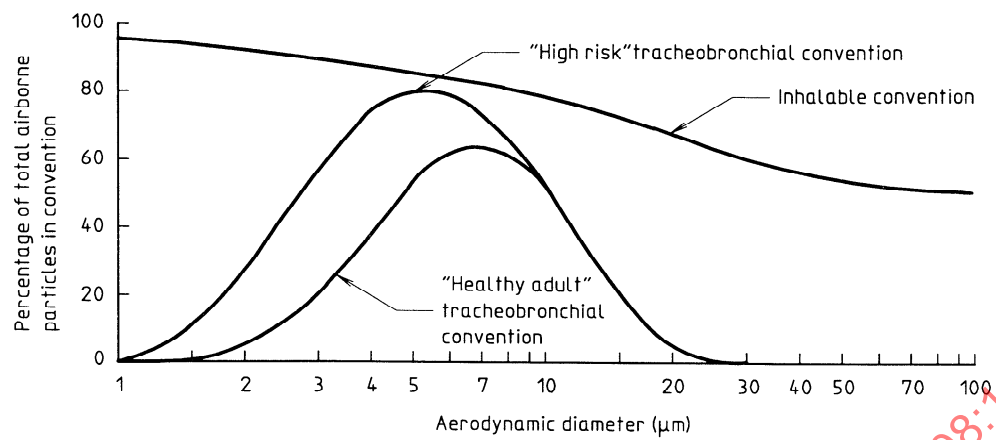
Figure B.2 — The tracheal and tracheobronchial conventions expressed as percentages of total airborne particulates
