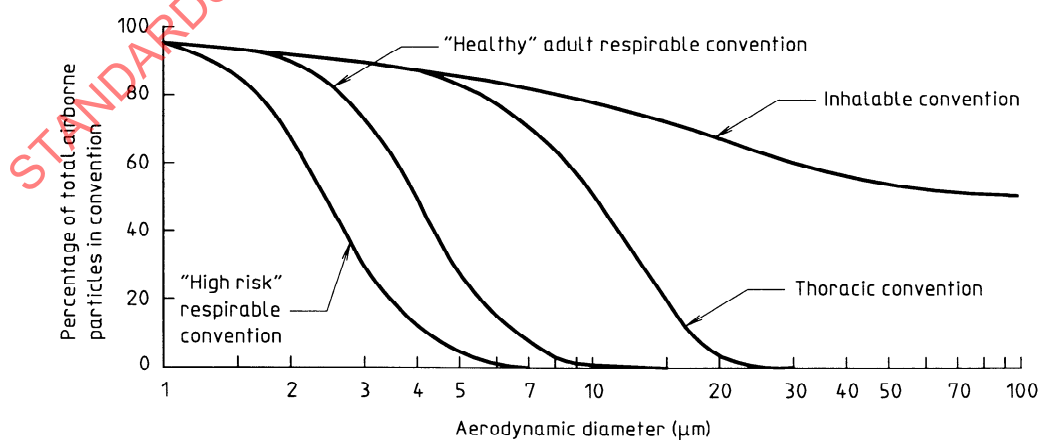
Figure B.1 — The inhalable, thoracic and respirable conventions expressed as percentages of total airborne particles
