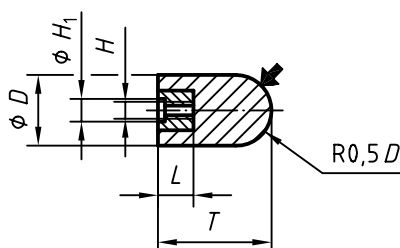
Figure 5 — Type 18R
