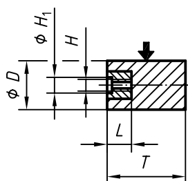
Figure 4 — Type 18
