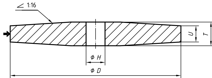
Figure 2 — Type 4
