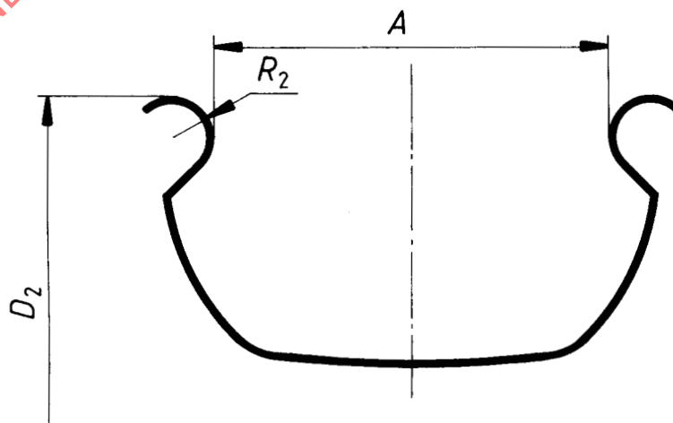
Figure 5 — Hooked bead rims
