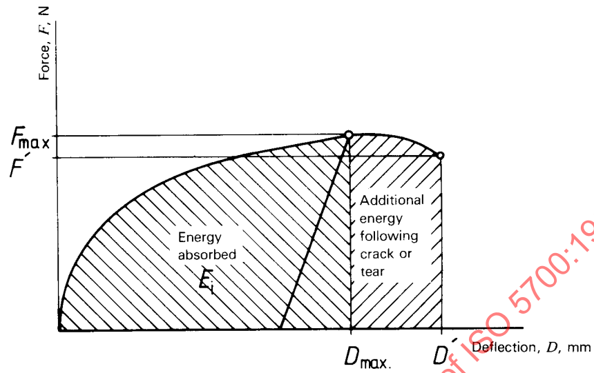
Figure 1 — Force-deflection ( F-D ) curve
