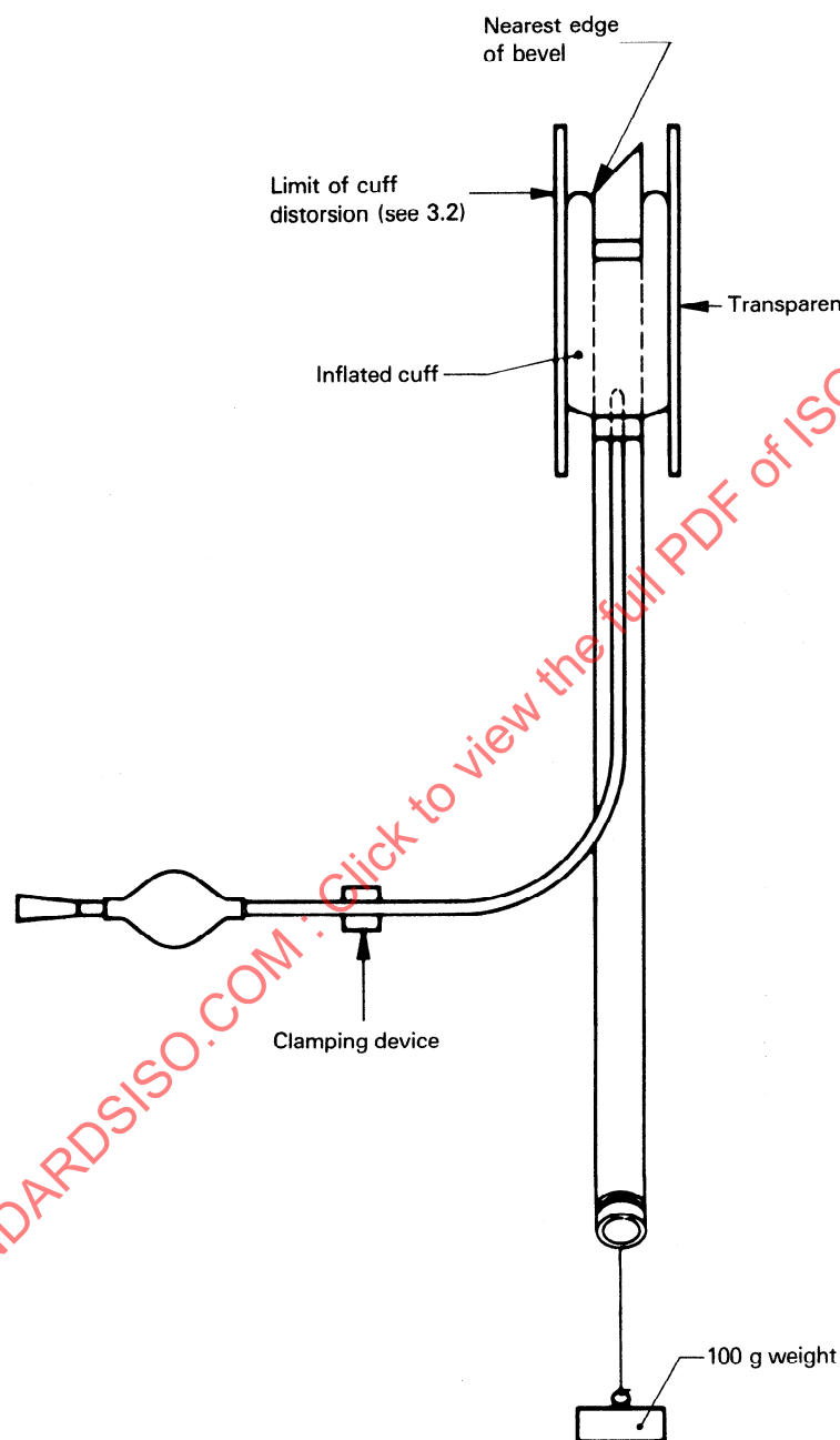
Figure 2 — Cuff herniation test (see 7.3 and 7.4)
