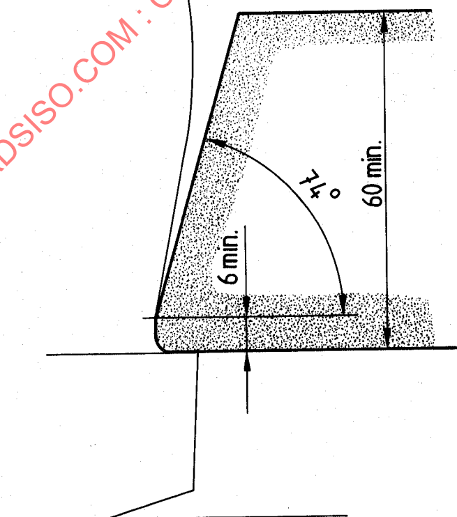
Figure 3 — Free space for the ski binding at the boot heel
