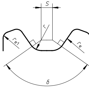
Figure 8 — Form of teeth on general purpose sprockets and key to tables 7 and 8
