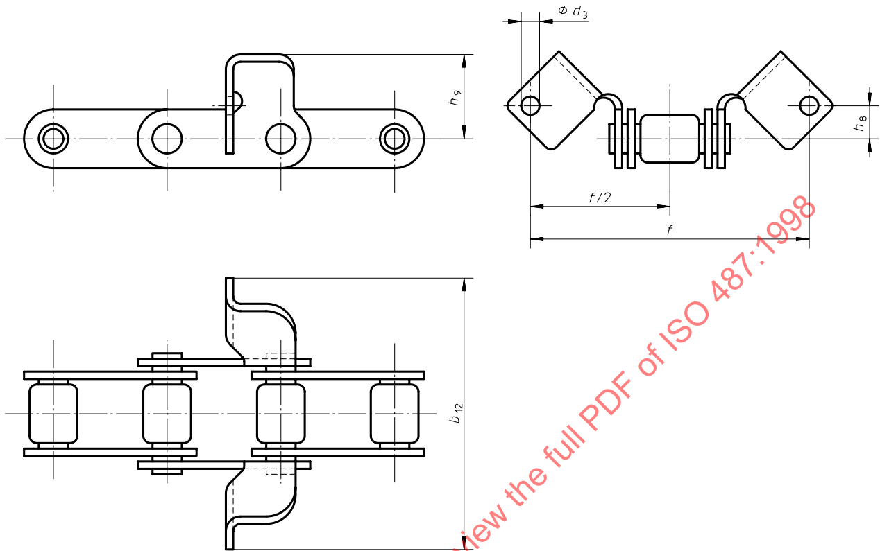
Figure 3 — F1 attachment plates
