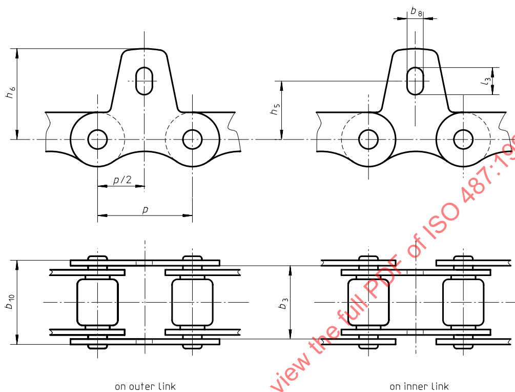
Figure 7 — M1 attachment plates
