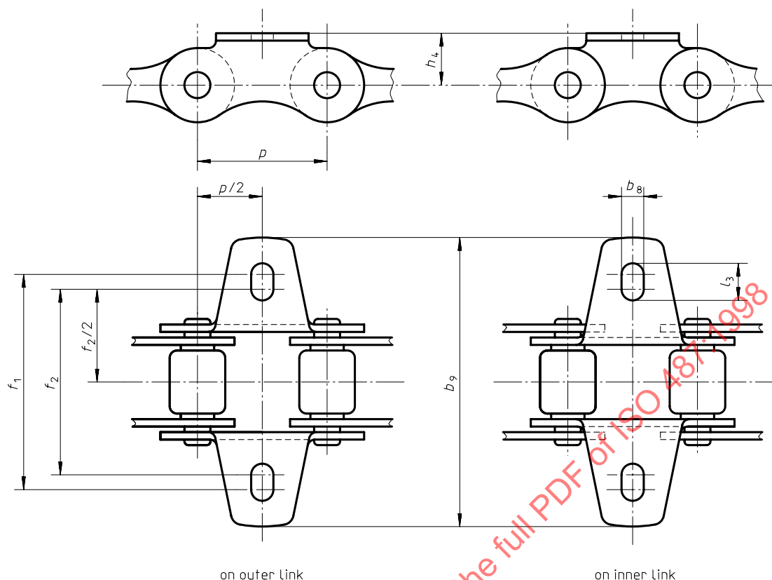
Figure 5 — K1 attachment plates for type S chains
