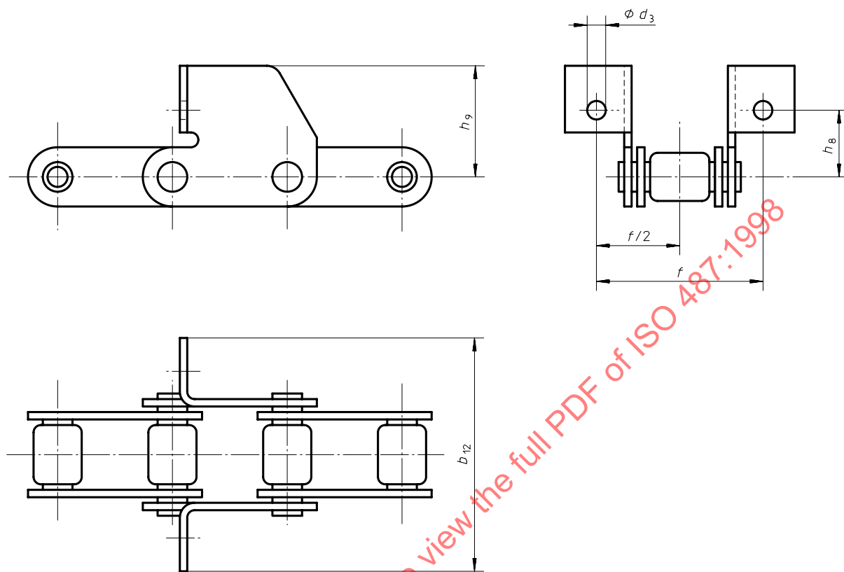
Figure 4 — F4 attachment plates
