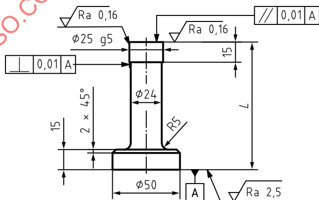
c) Lower punch, L = H + 35
