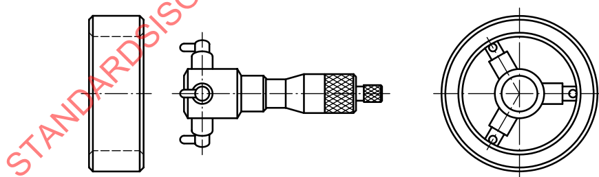
Figure 4 — Three-point measuring instrument
