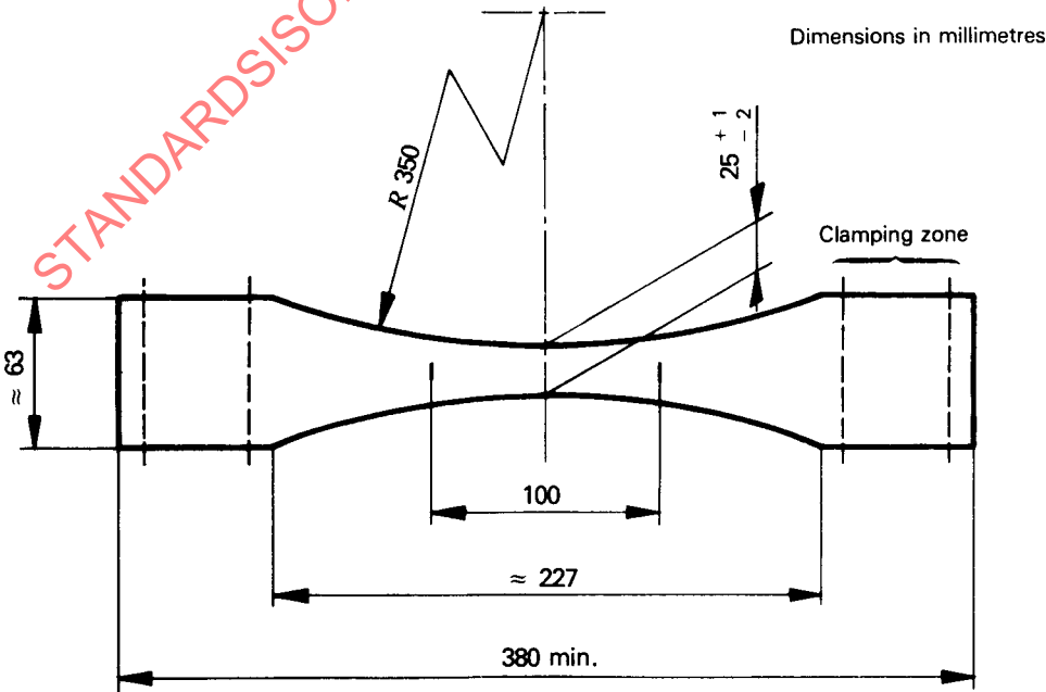
Figure 5 — Type C test piece
