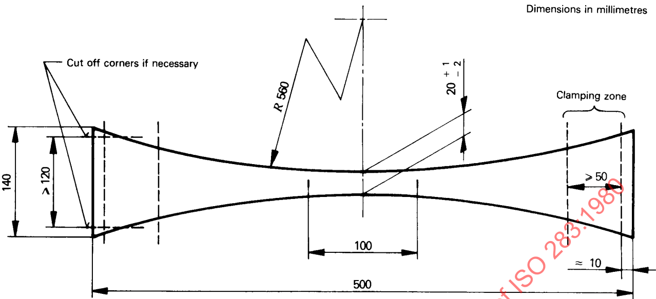
Figure 4 — Type B test piece
