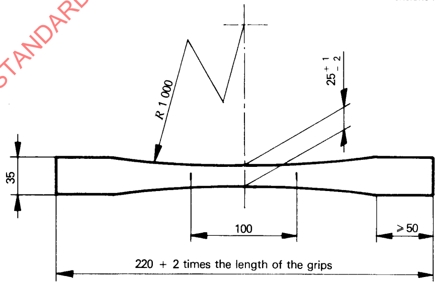
Figure 3 — Type A test piece
