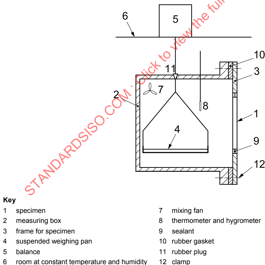
Figure 1 — Test apparatus
