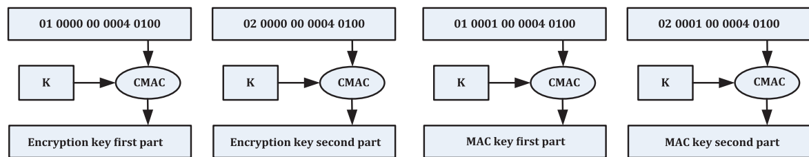
Figure 4 — Deriving 256-bit AES MAC and CBC encryption keys
