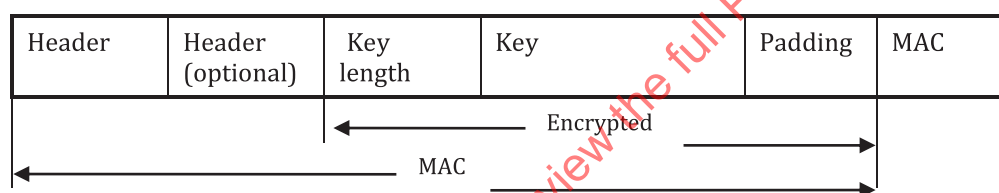
Figure A.1 — CBC MAC Key Block
