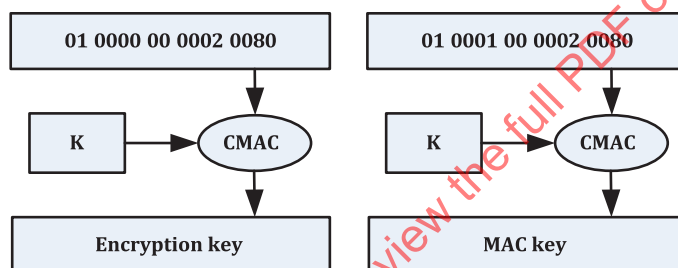
Figure 2 — Deriving AES 128 MAC and CBC encryption keys
