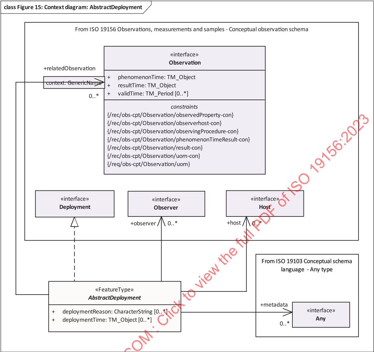
Figure 15 — Context diagram for Abstract Observation Core — AbstractDeployment
