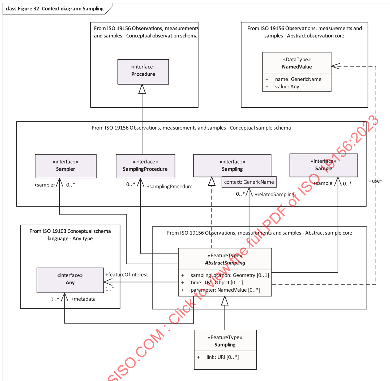
Figure 32 — Context diagram for Basic Samples — Sampling
