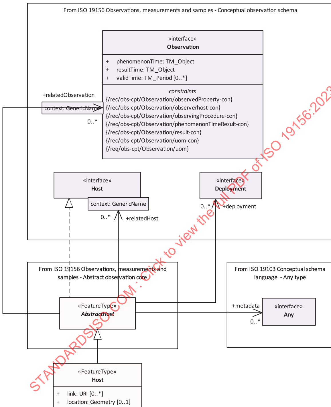
class Figure 22: Context diagram: Host
