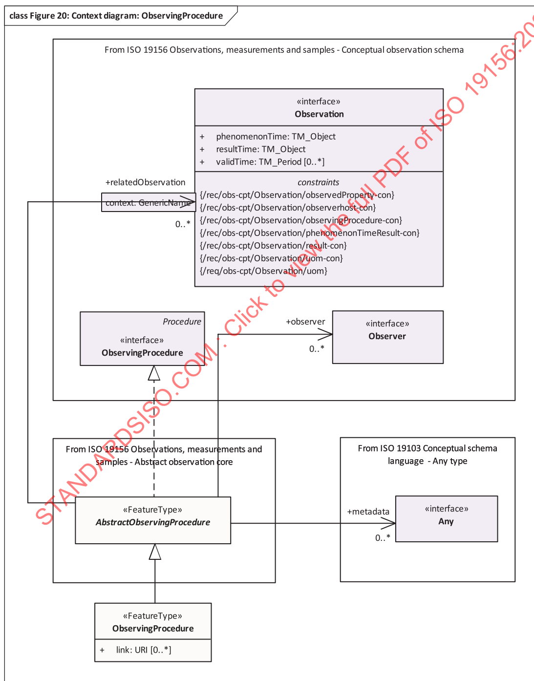
Figure 20 — Context diagram for Basic Observations — ObservingProcedure
