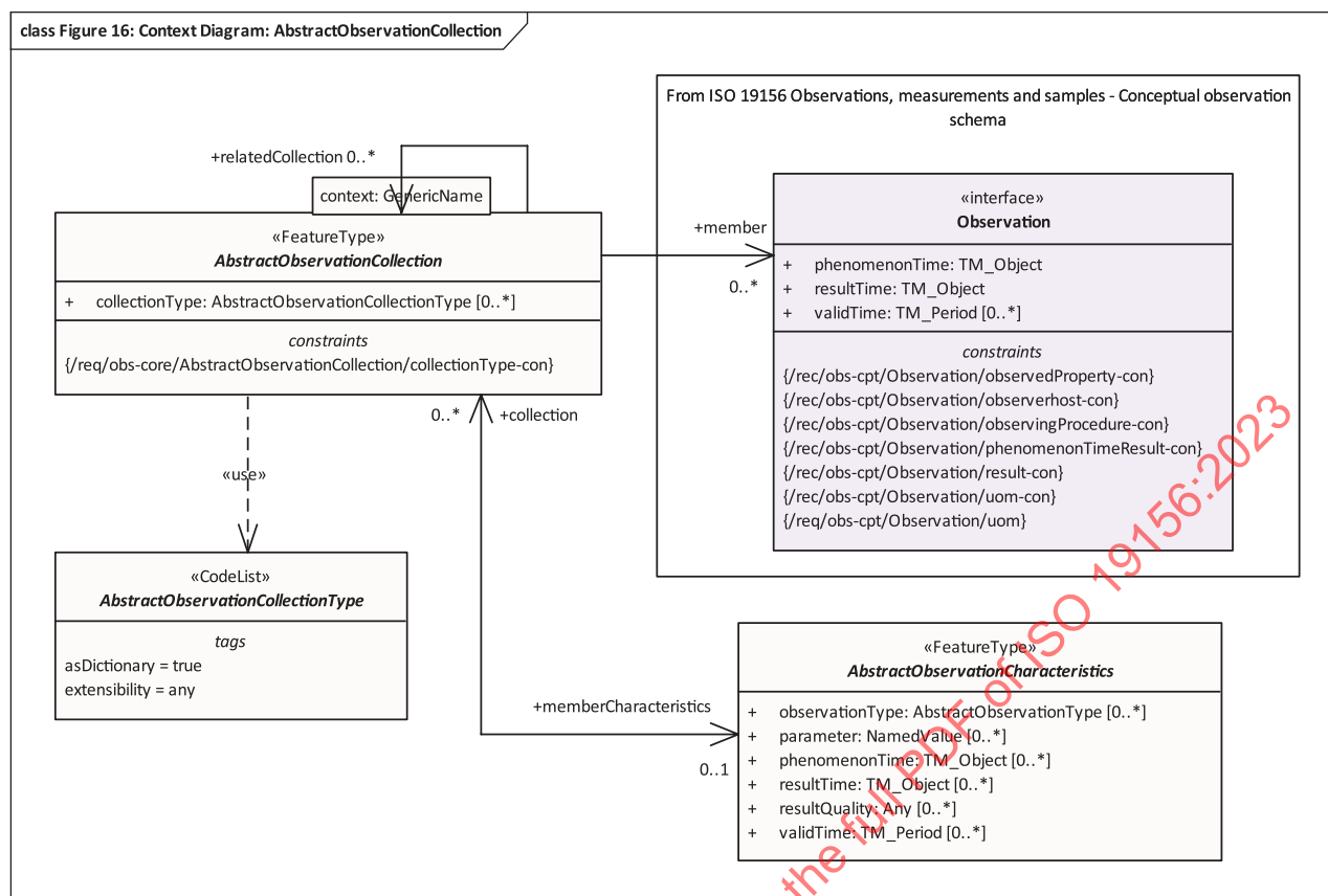
Figure 16 — Context diagram for Abstract Observation Core — AbstractObservationCollection
