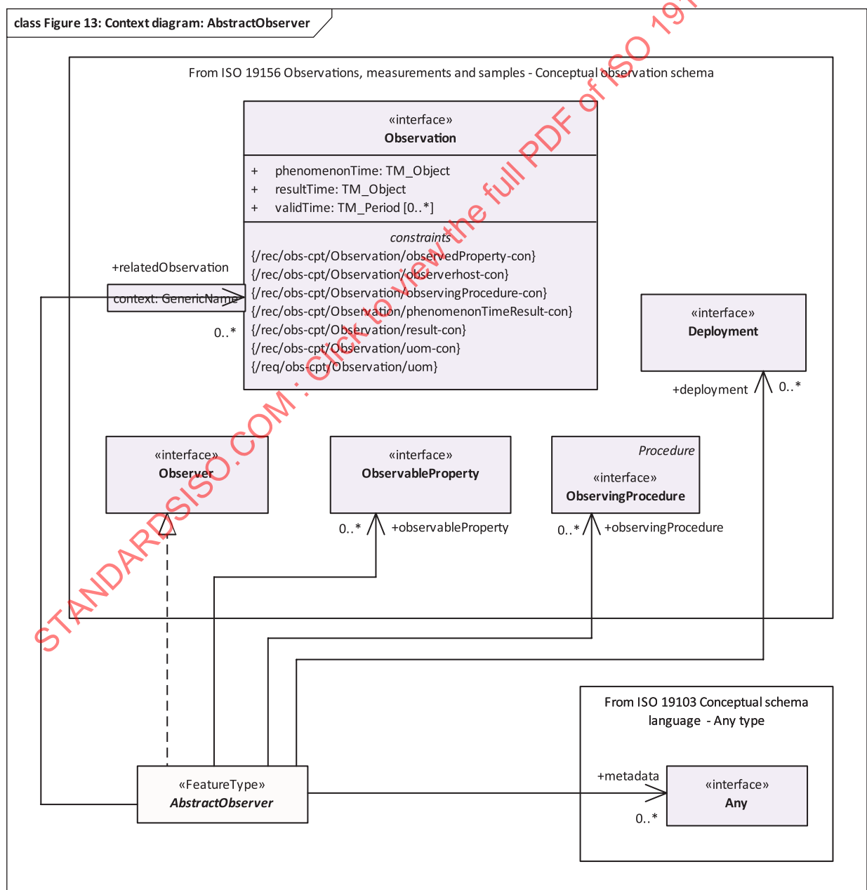
Figure 13 — Context diagram for Abstract Observation Core — AbstractObserver
