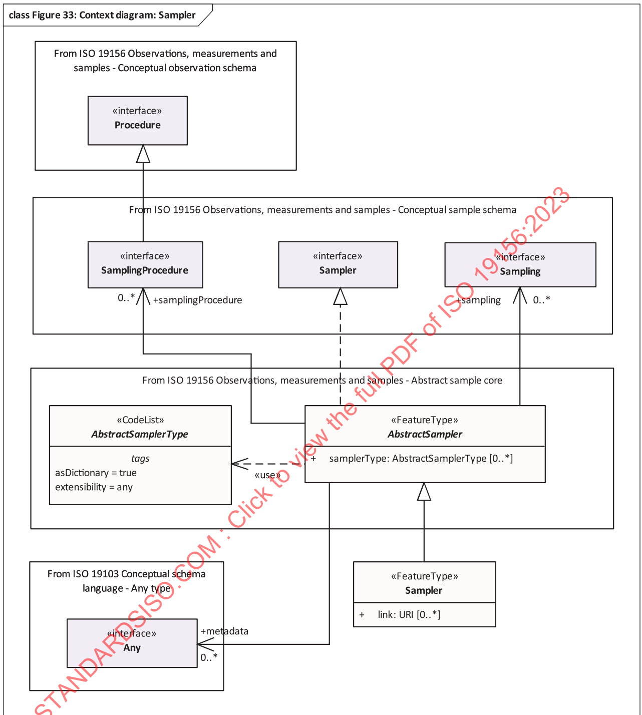
Figure 33 — Context diagram for Basic Samples — Sampler
