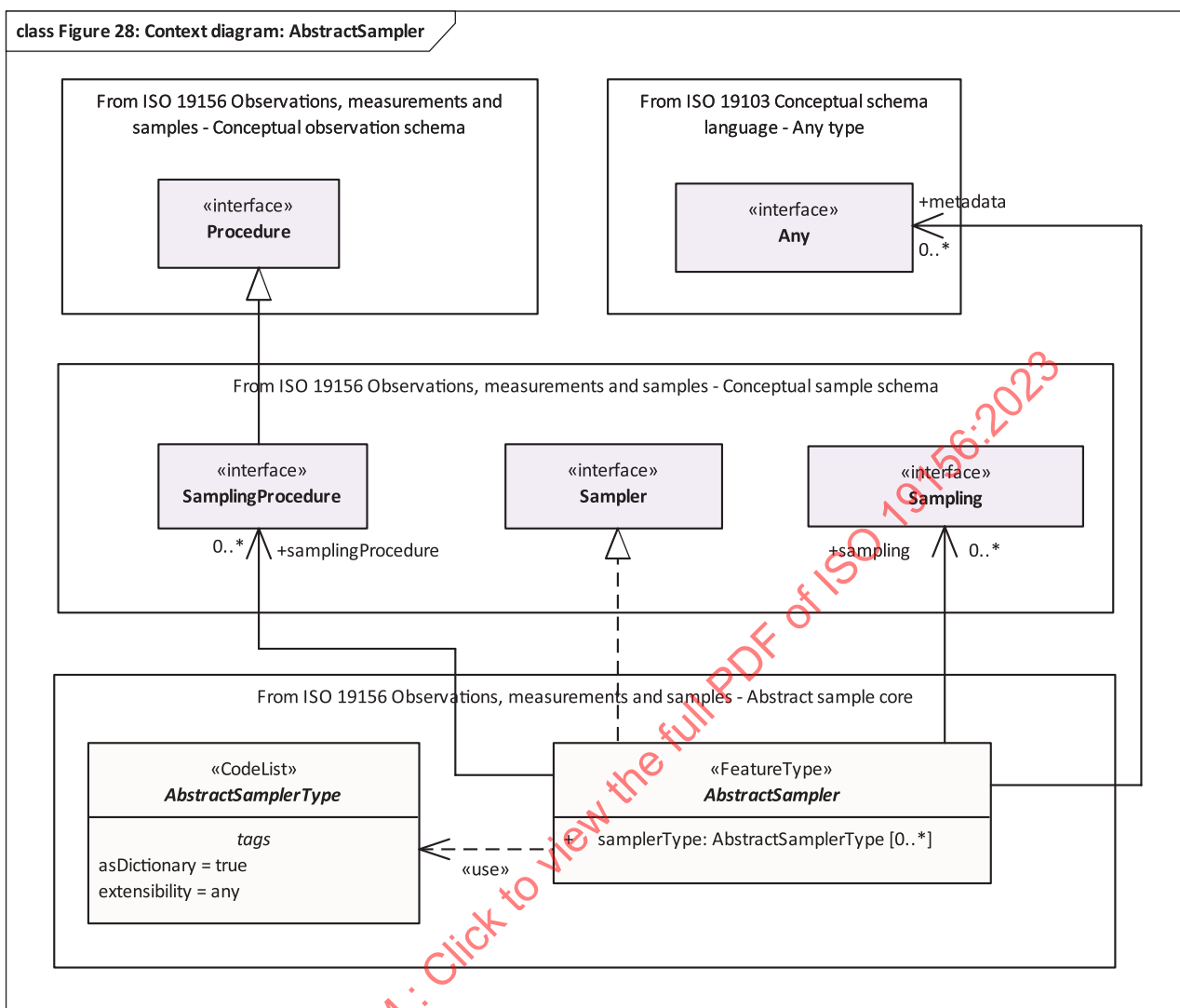
Figure 28 — Context diagram for the Abstract Sample Core — AbstractSampler
