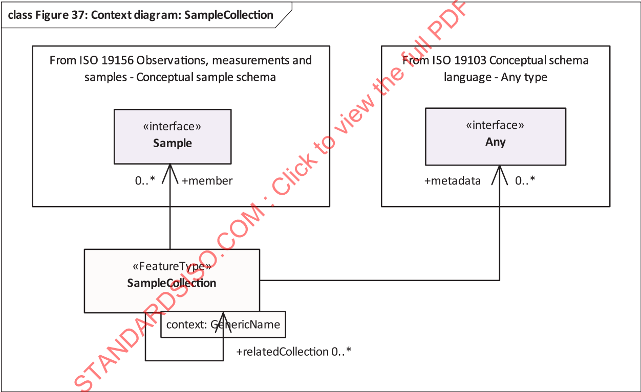
Figure 37 — Context diagram for Basic Samples — SampleCollection
