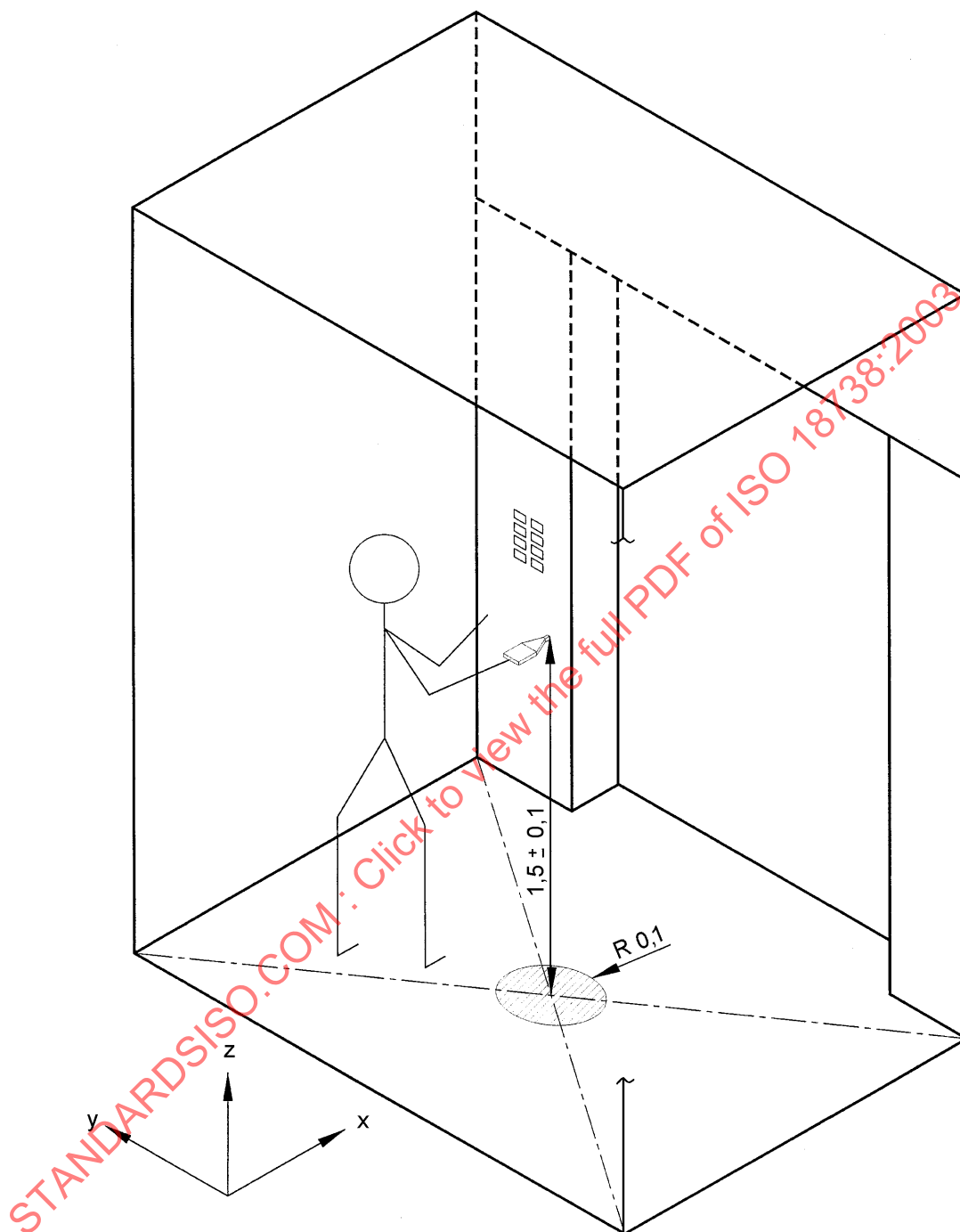
Figure 10 — Location of transducers
