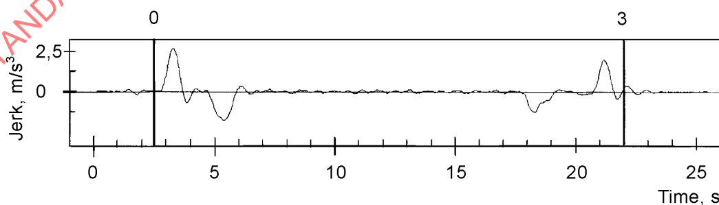
Figure 4 — Jerk signal
