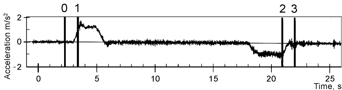
Figure 1 — Boundaries of calculation shown on a typical z -axis acceleration signal
