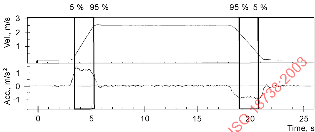
Figure 3 — Calculation of A95 acceleration and deceleration
