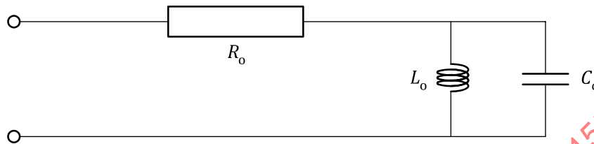
Figure 1 — Excitation-element impedance
