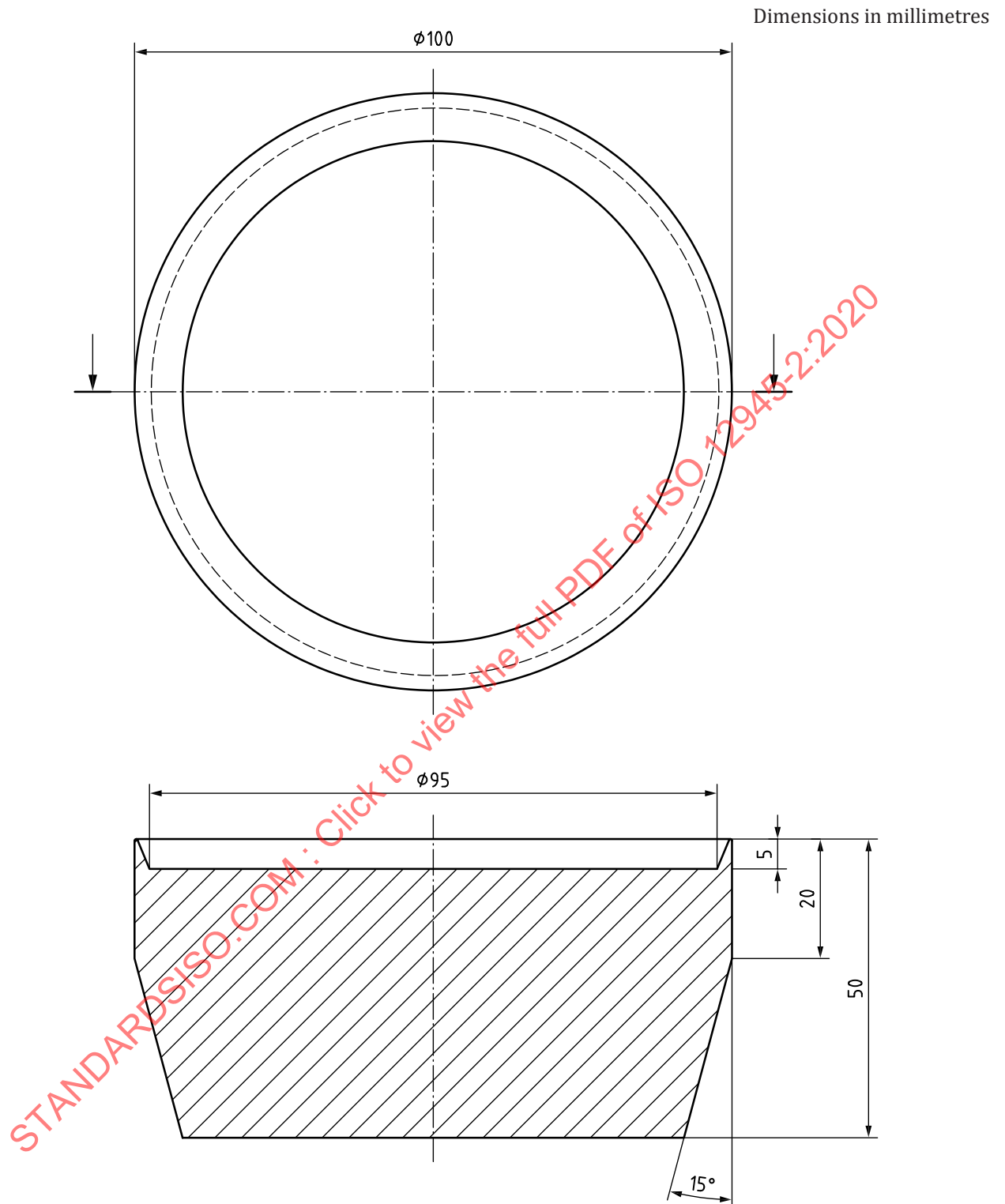
Figure 5 — Auxiliary device for test specimen mounting
