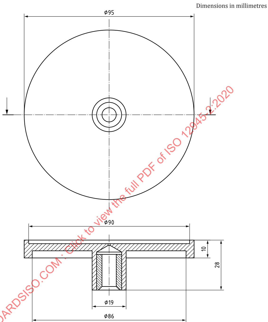
Figure 3 — Test specimen holder body
