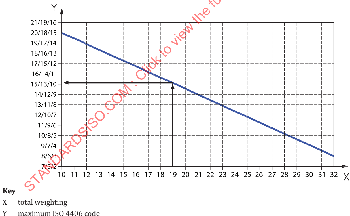
Figure 1 — Relationship of total weighting and ISO 4406 codes used to derive the required cleanliness level (RCL)
