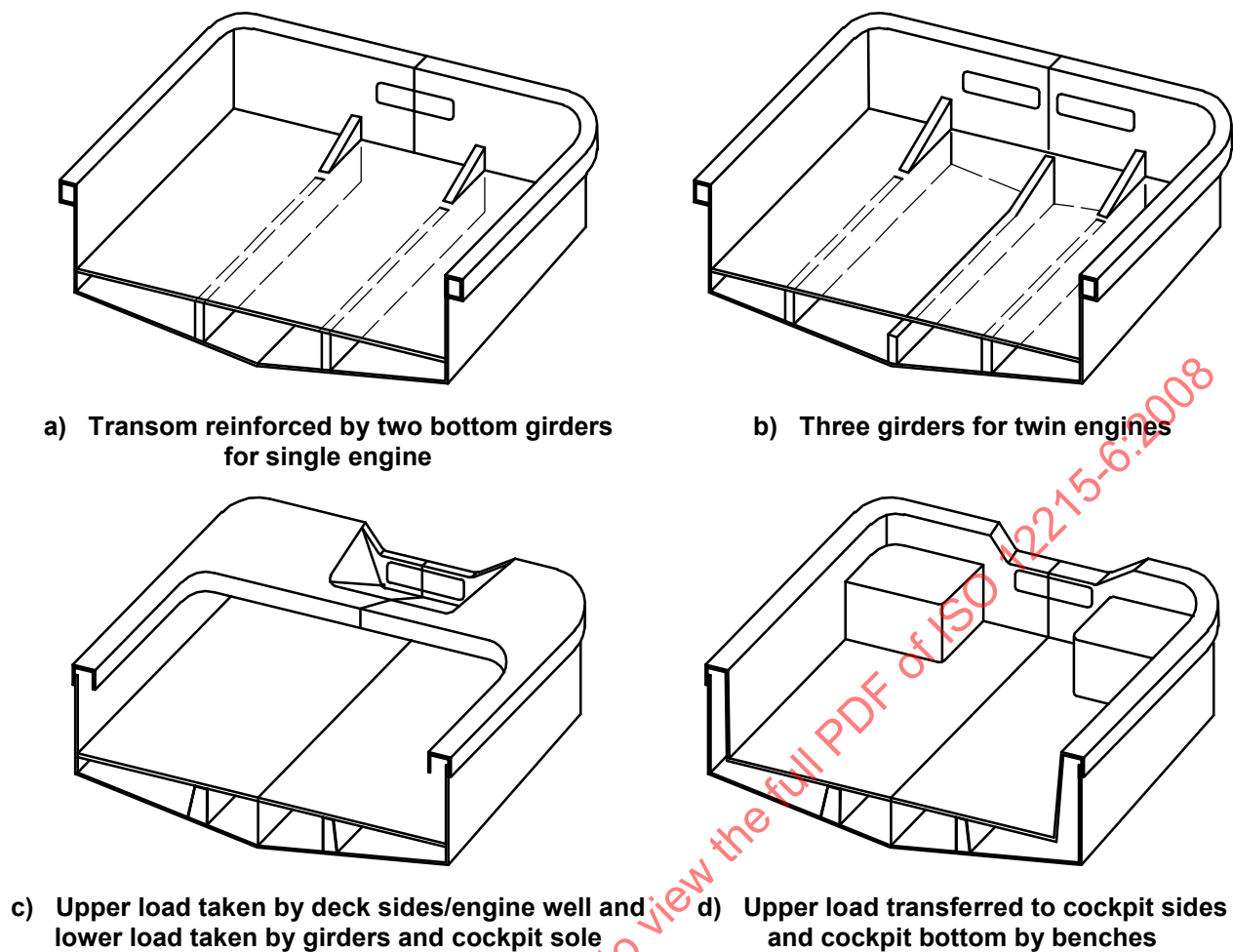
Figure 15 — Examples of transom configuration
