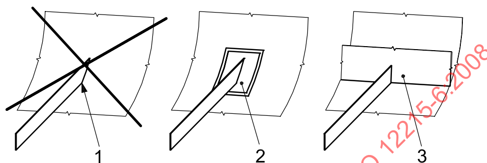
a) Stiffener ending in shell, poor practice and good practice
