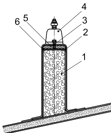
a) Typical mounting on top of foam or plywood former
