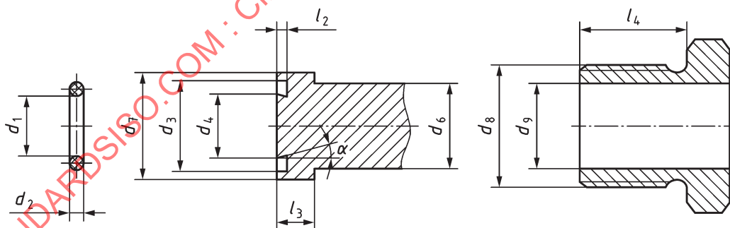
Figure 20 — 500 bar plug connection — Parts
