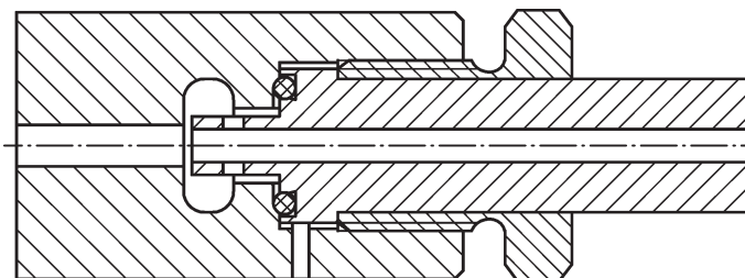
Figure 15 — 500 bar filling connection — Assembly drawing
