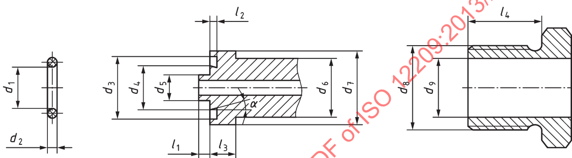
Figure 18 — 500 bar gas withdrawal connection — Parts
