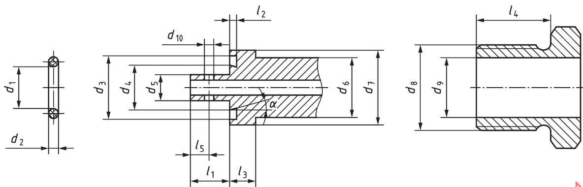
Figure 16 — 500 bar filling connection — Parts
