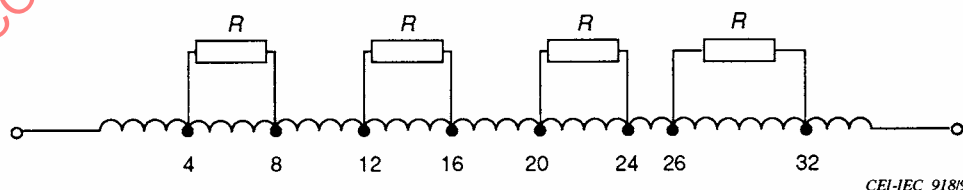
Figure A.3 – Schematic of 50 \mu H inductor
