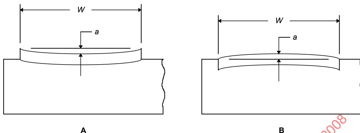
Figure 1 — Surface profile
