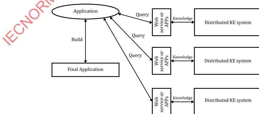
Figure 5 — KE distribution architecture
