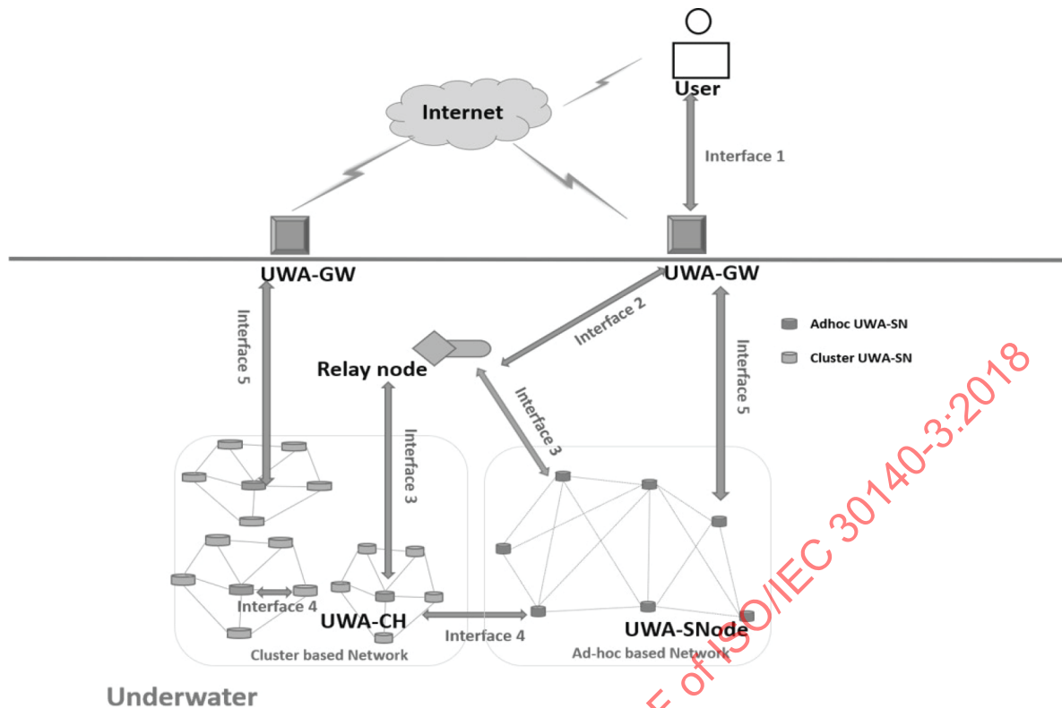
Figure 3 – Interfaces between physical entities
