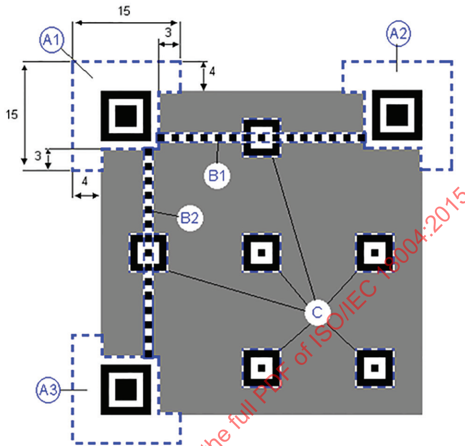
Figure G.1— QR Code fixed pattern segments
