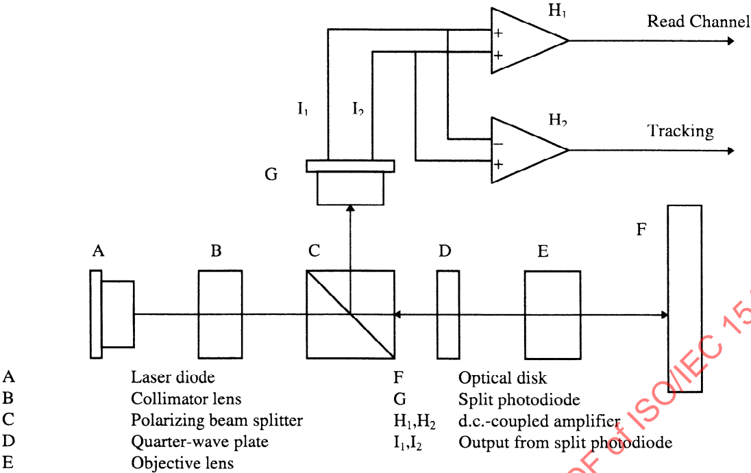
Figure 1 - Optical system of the Reference Drive
