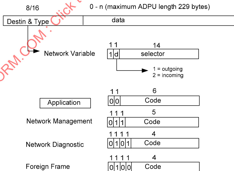
Figure 30 — APDU format
