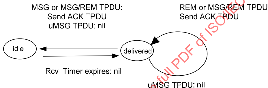
Figure 19 — Transport protocol—Receive FSM
