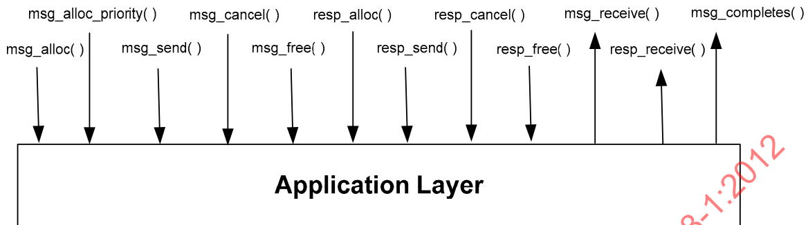
Figure 29 — Application layer interface
