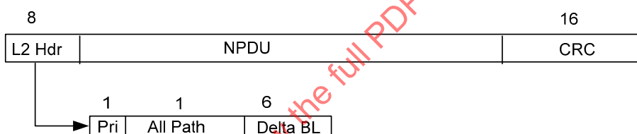
Figure 5 — MPDU/LPDU format
