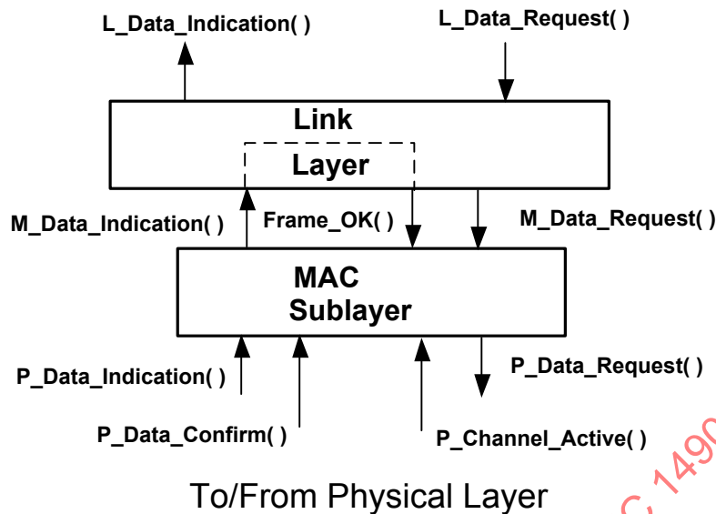
Figure 4 — Interface between the MAC and the link layers
