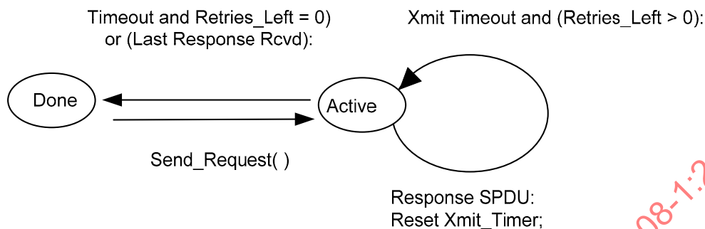
Figure 27 — Request-response protocol—client FSM
