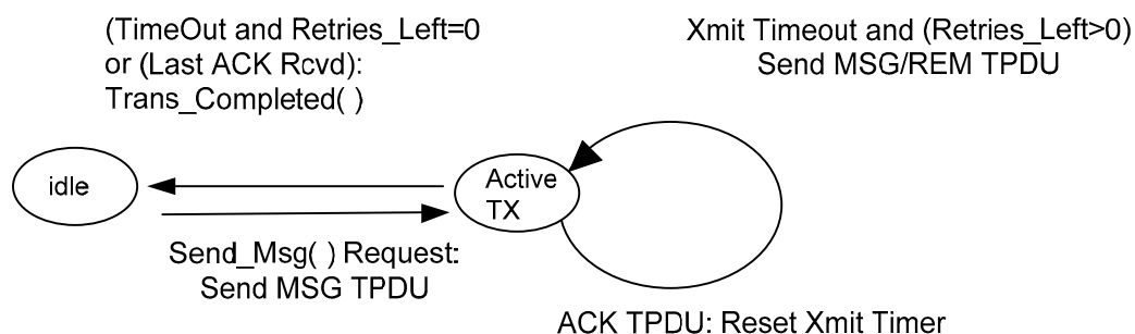
Figure 18 — Transport protocol—Send FSM
