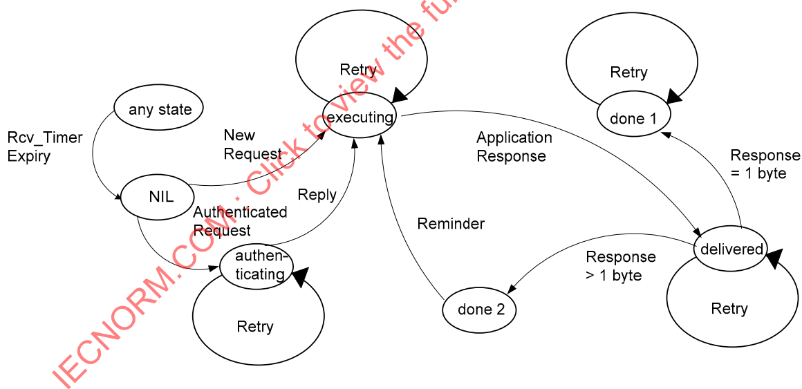
Figure 28 — Request-response protocol—simplified server FSM
