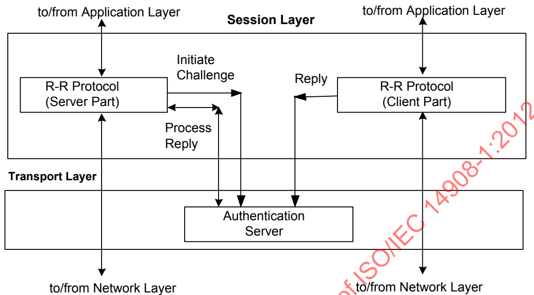
Figure 23 — Session layer—internal structuring
