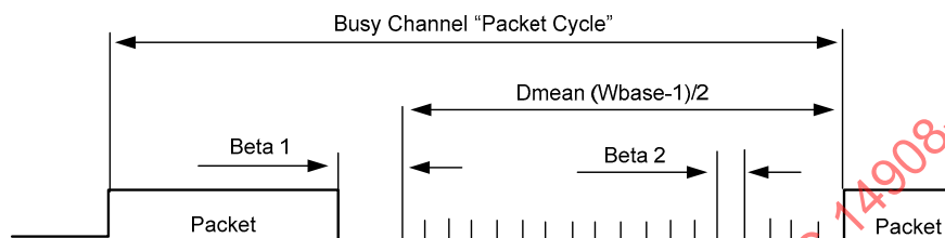
Figure 6 — Predictive p -persistent CSMA concepts and parameters
