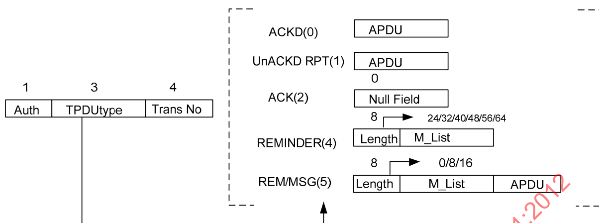
Figure 16 — TPDUs and formats
