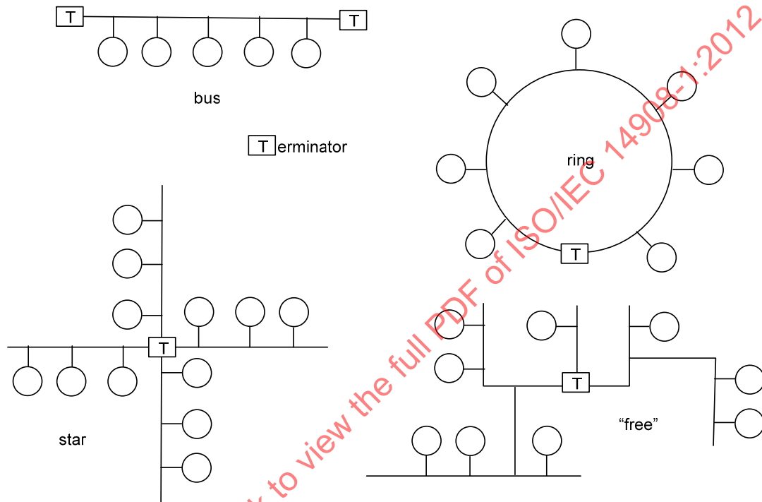
Figure 9 — Single channel topologies
