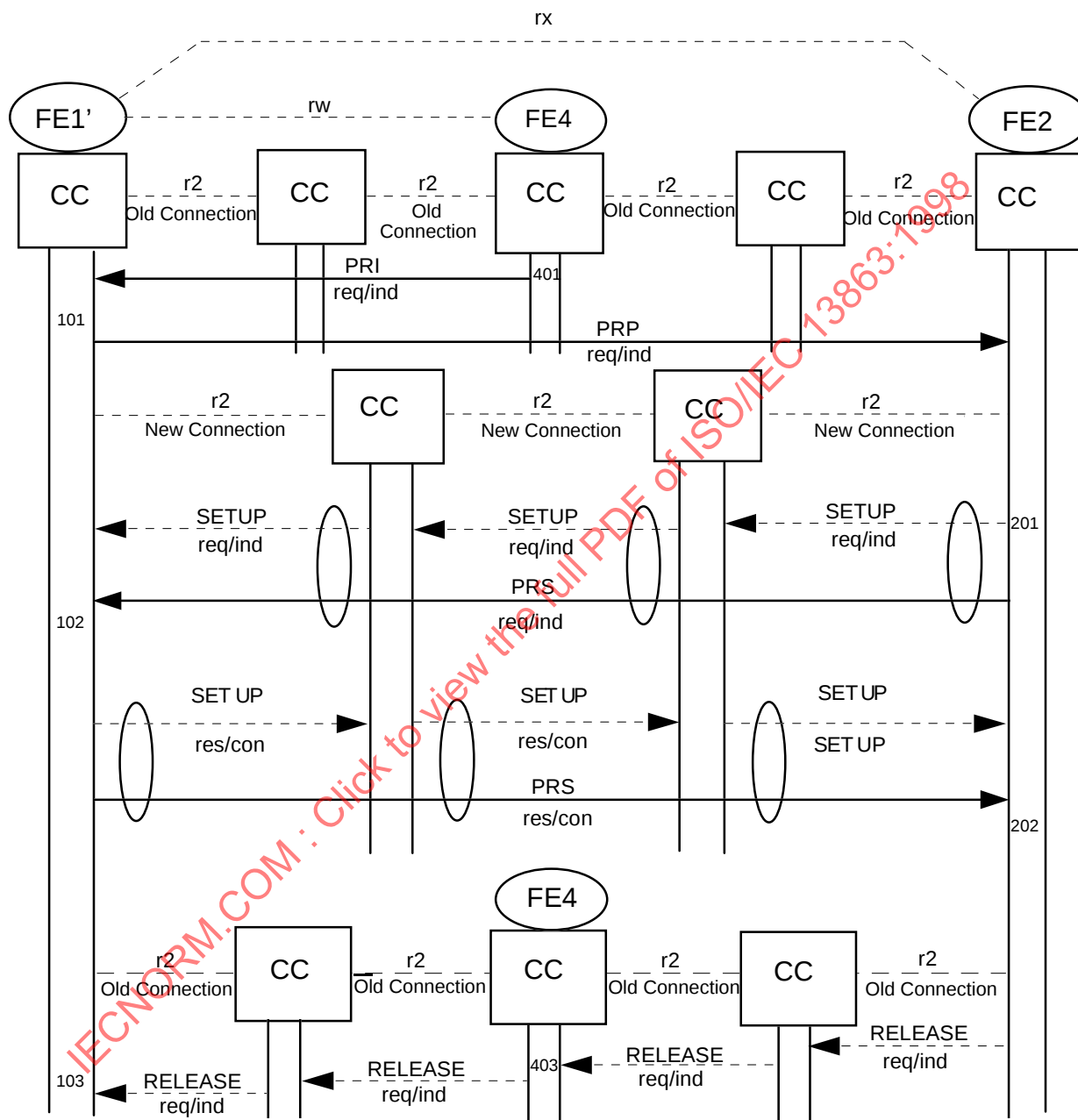
Figure 17 - Information flow sequence - normal operation of ANF-PR
