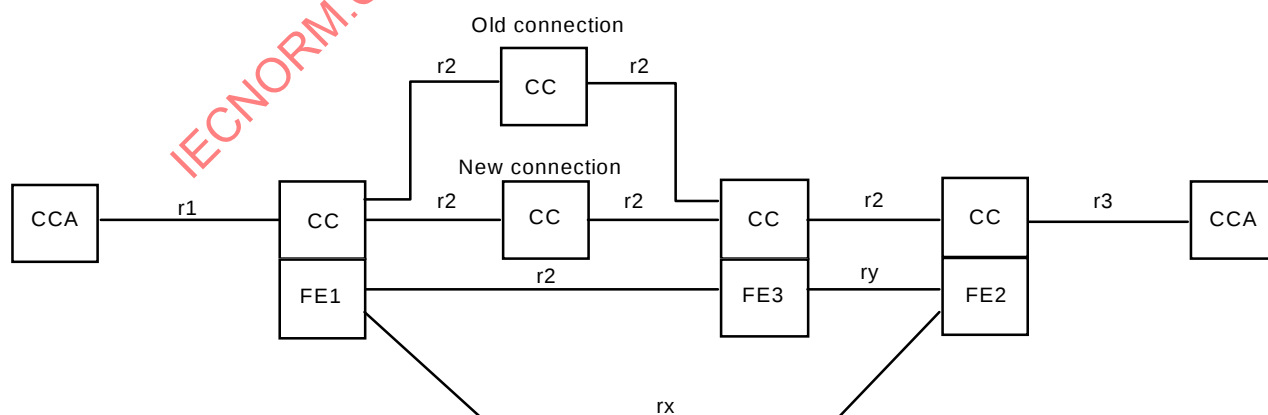
Figure 9 - Example relationship between models for ANF-PR and basic call - re-use of part of the old connection
