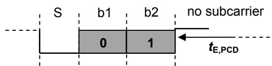
Figure Amd.2.3 — Test pattern for the EMD recovery test (Type A)
