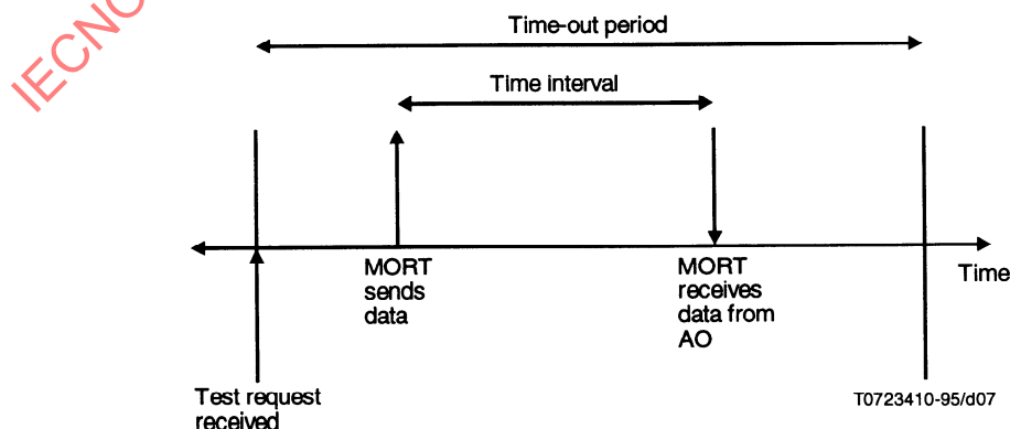
Figure 7 – Data integrity test example 1
