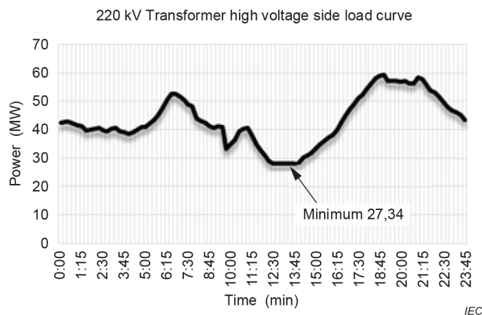
Figure D.2 – Operation data of typical day
