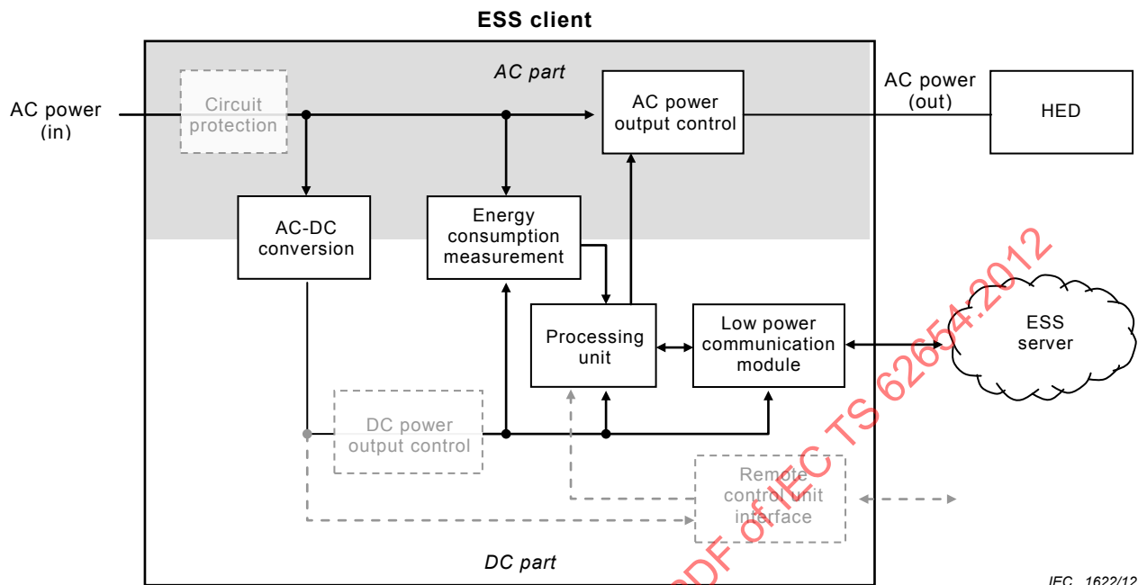
Figure 3 – Basic architecture of ESS client
