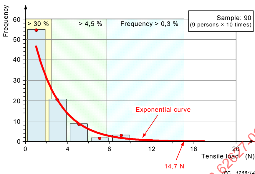
Figure 3 – Tensile load histogram
