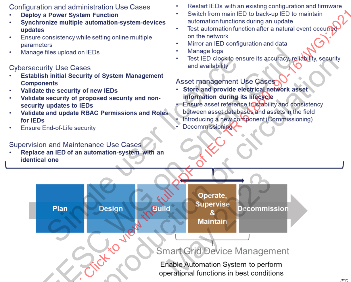
Figure 3 – Different Use Cases through the lifecycle of a smart grid system
