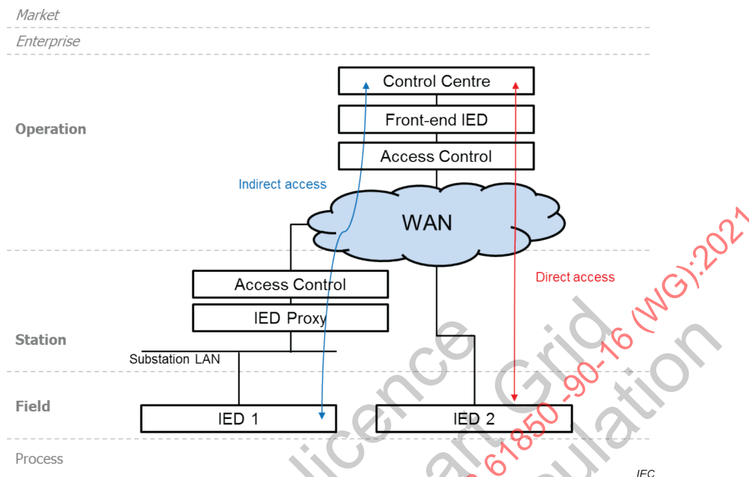
Figure 5 – Interactions between Information System and IEDs
