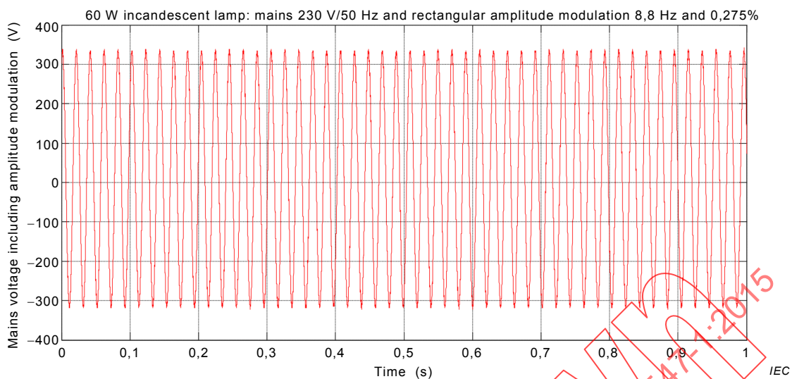
a) Mains voltage fluctuation with rectangular modulated of 8,8 Hz and \lambda = 0,275\%
