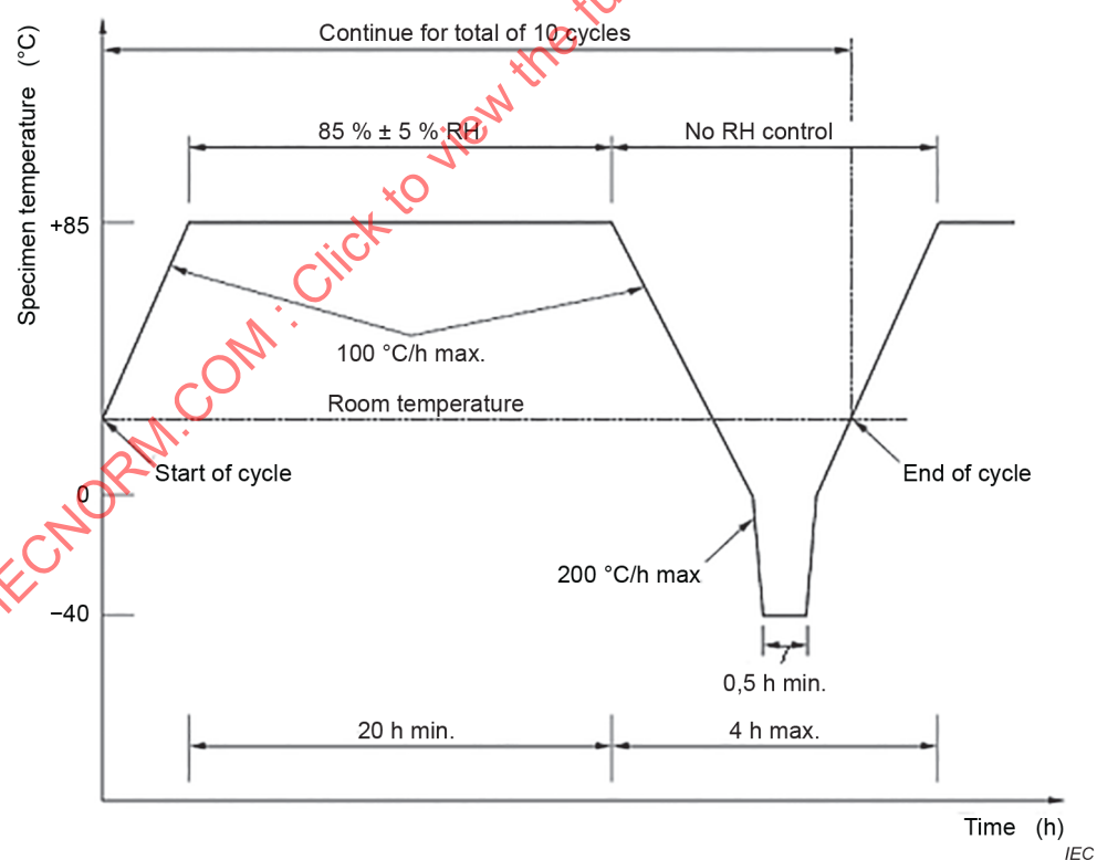
Figure 2 – Humidity-freeze cycle
