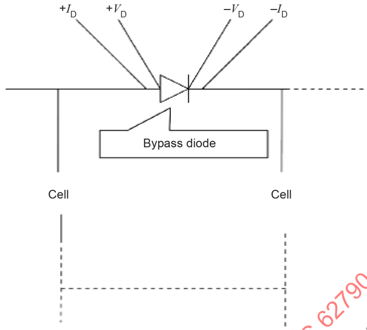
Figure 7 – Bypass diode thermal test
