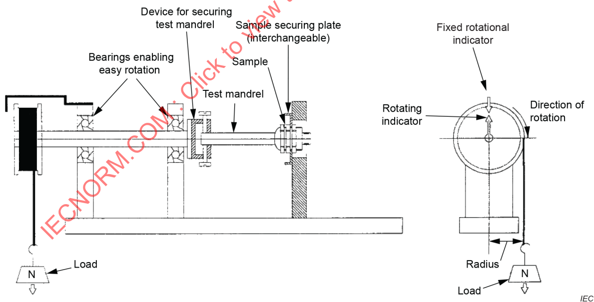
Figure 4 – Typical arrangement for torsion test
