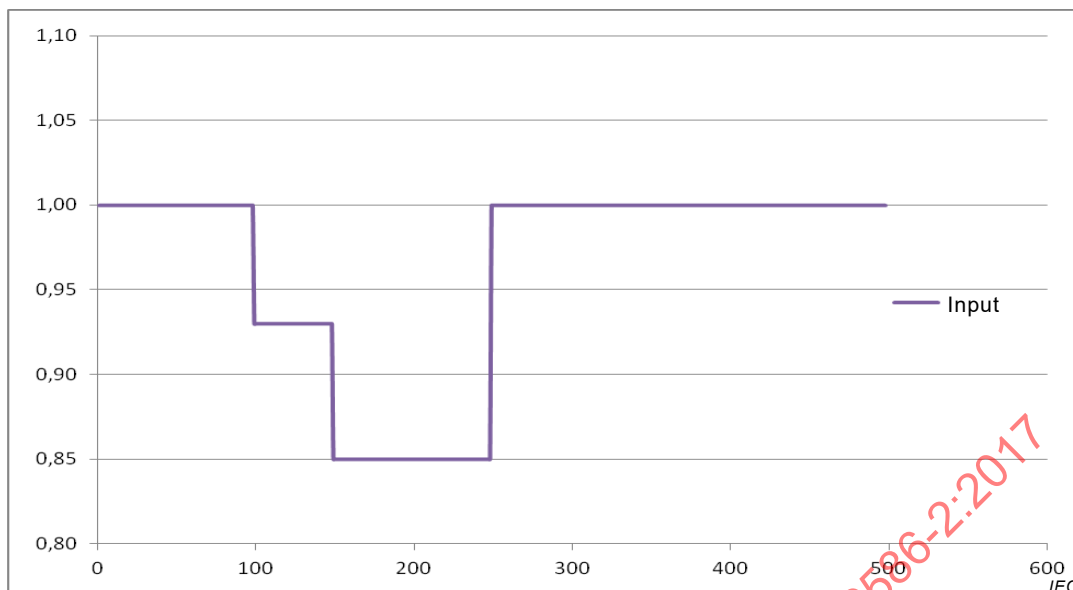
Figure 23 – A13.1.3 waveform
