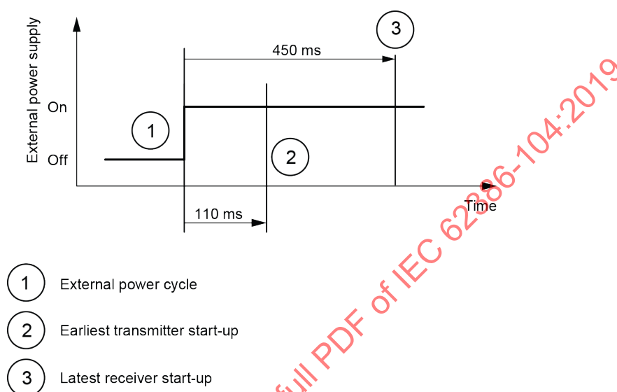
Figure 4 – Start up timing example
