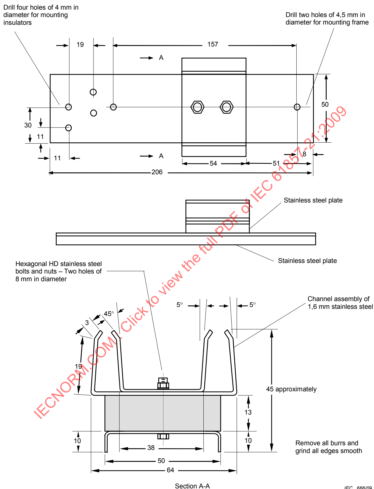
Figure 2 – Schematic drawing of a GPM frame
